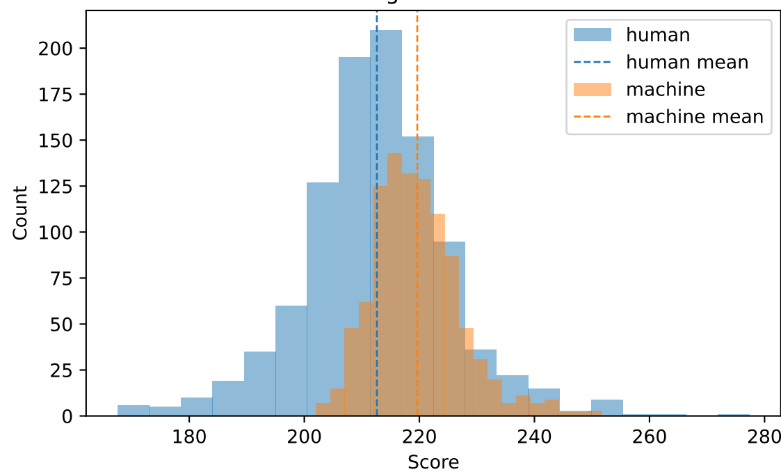
Length Std
