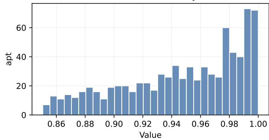
Semantic Similarity
