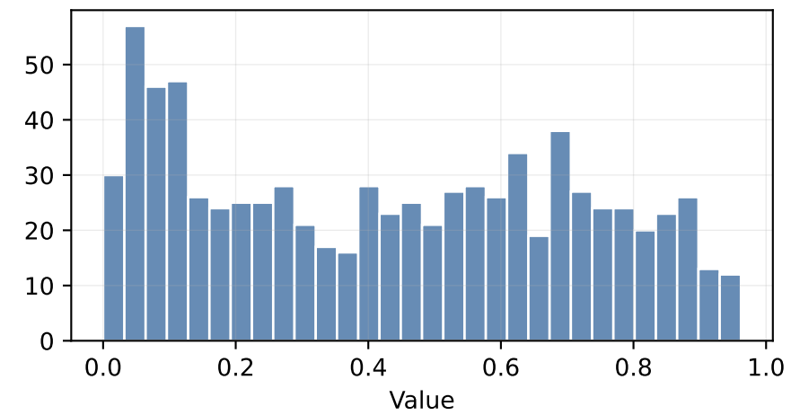
Levenshtein Distance
