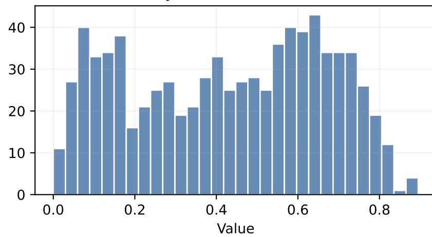
Jaccard Distance
