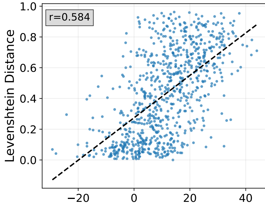
Projection Score
