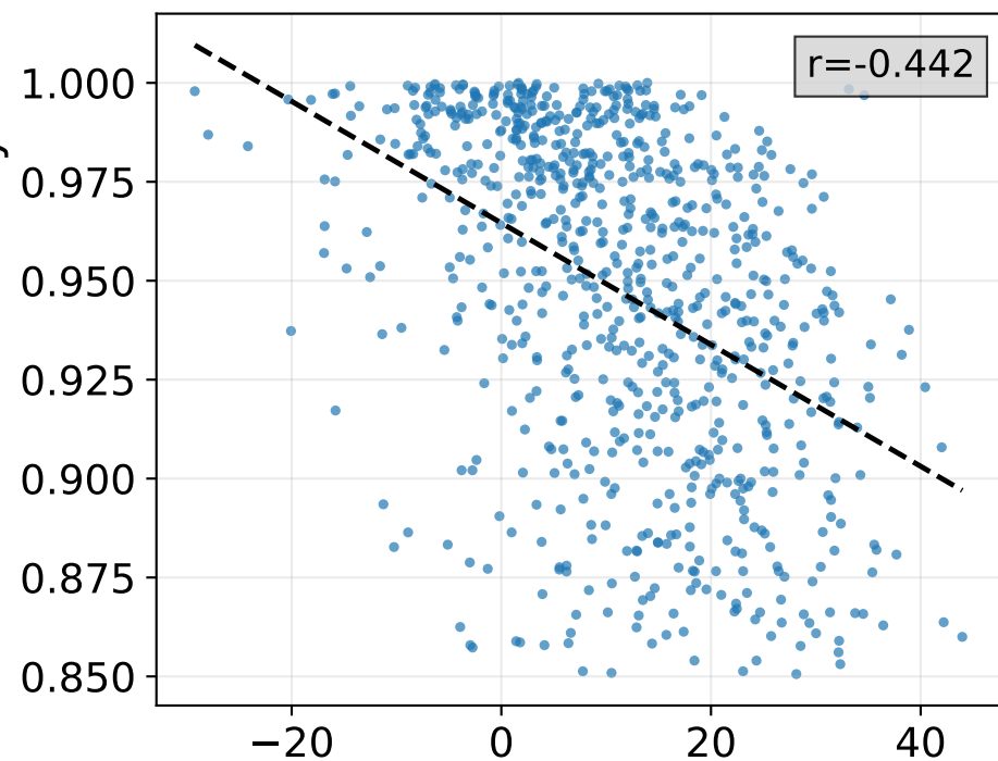
Levenshtein Distance
