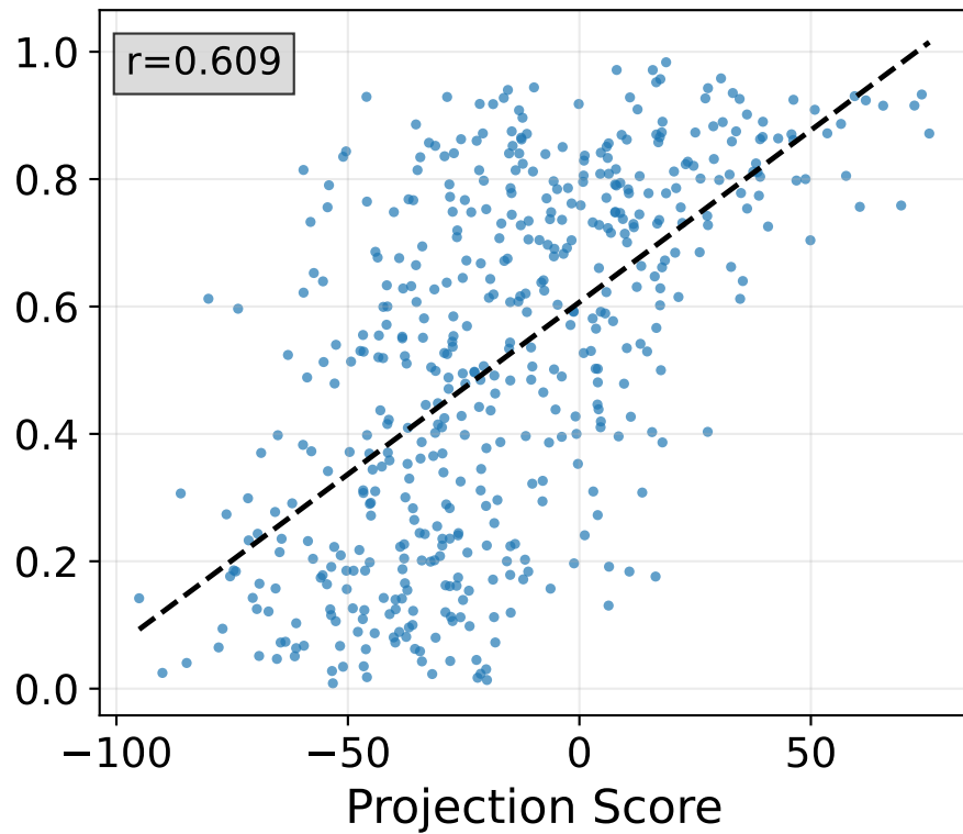
Levenshtein Distance
