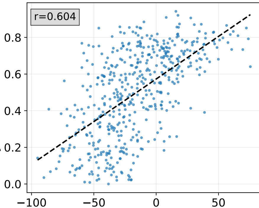
Jaccard Distance
