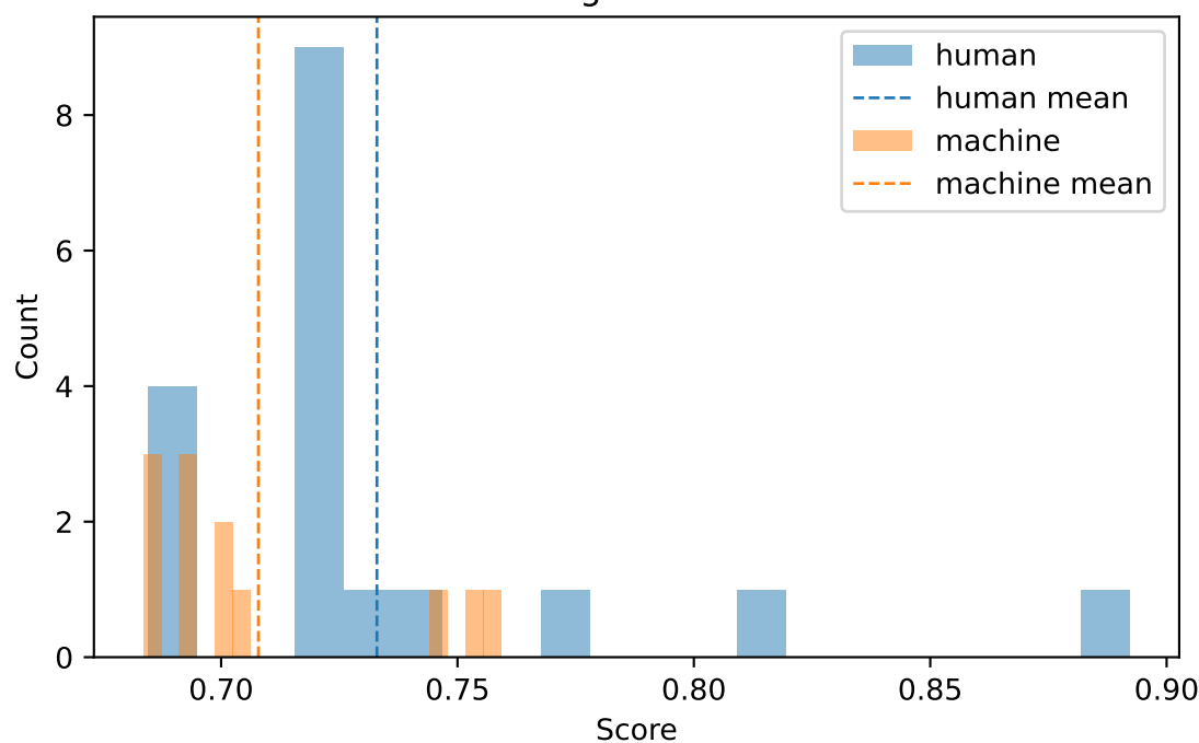
Magnitude Mean
