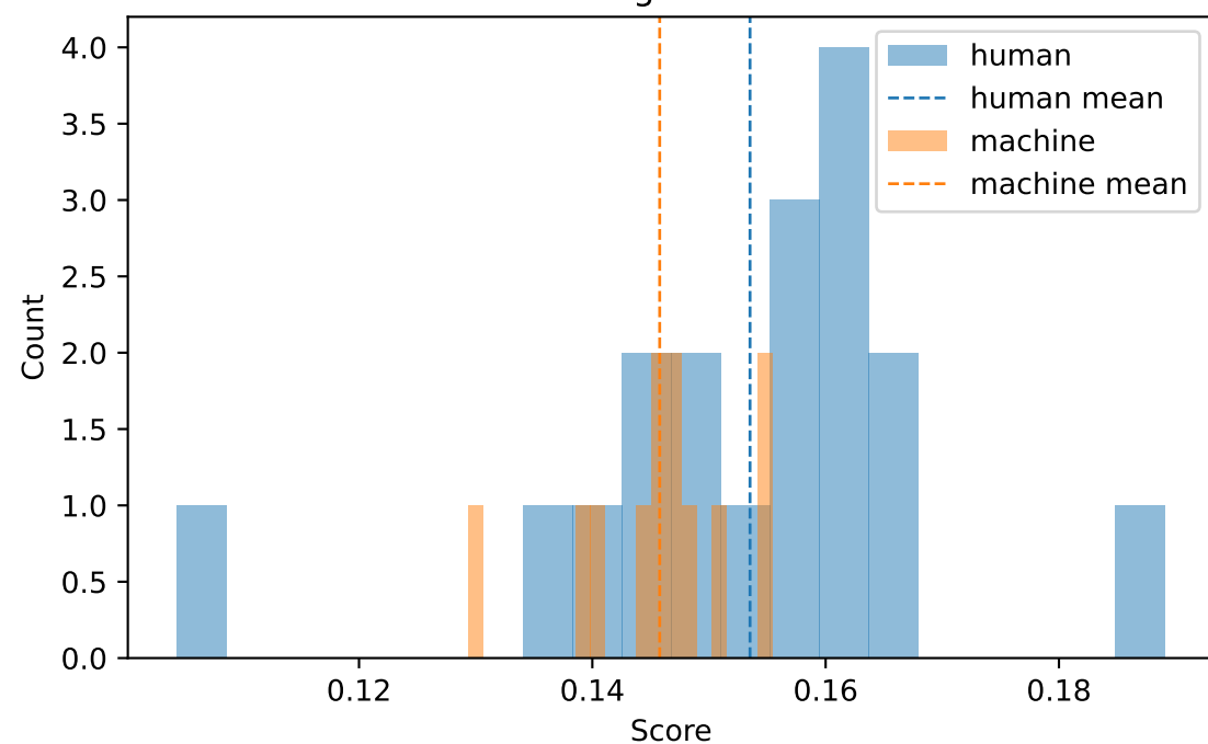
Magnitude Std
