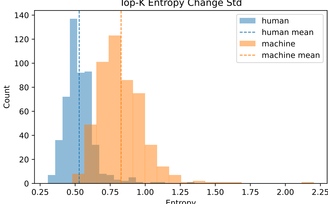
Top-K Entropy Change Std
