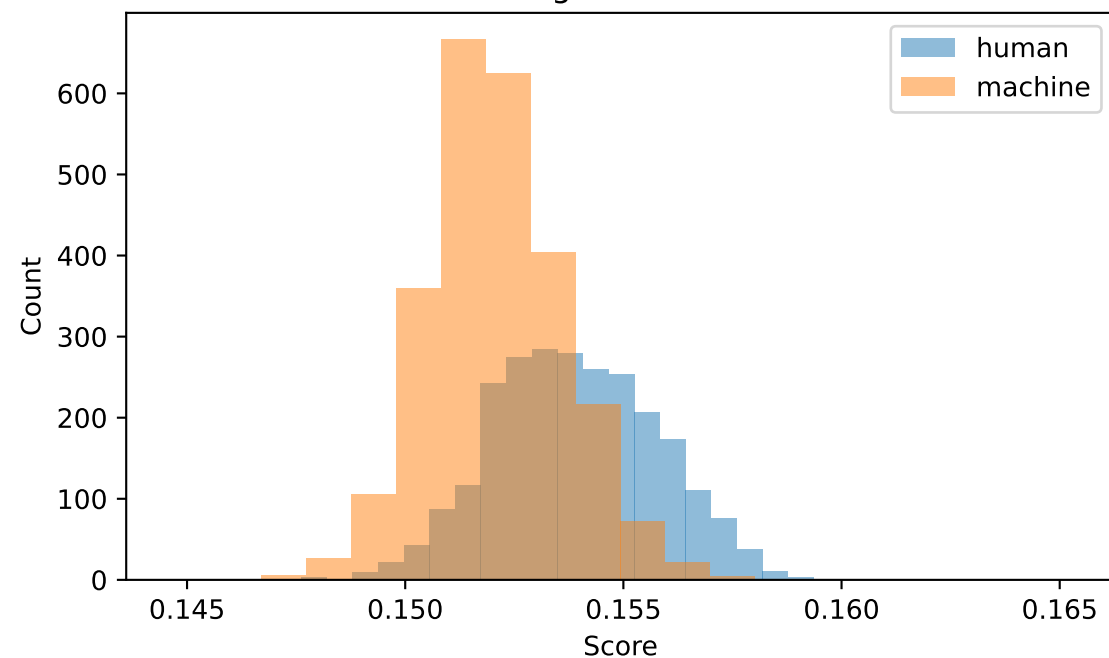
Magnitude Std
