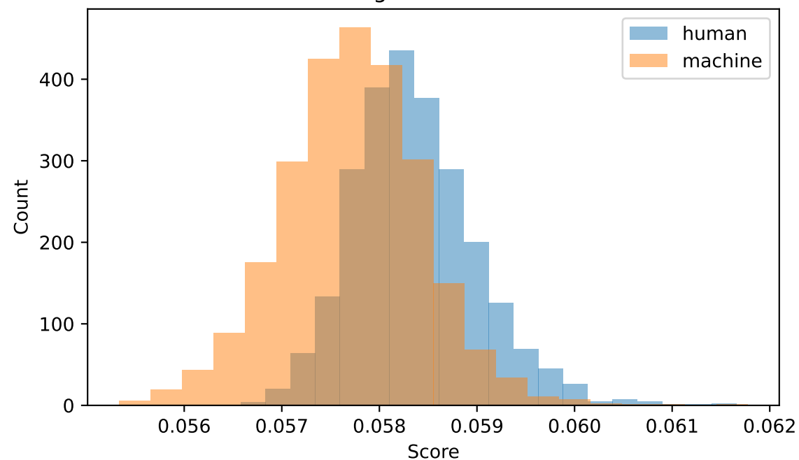
Magnitude Mean
