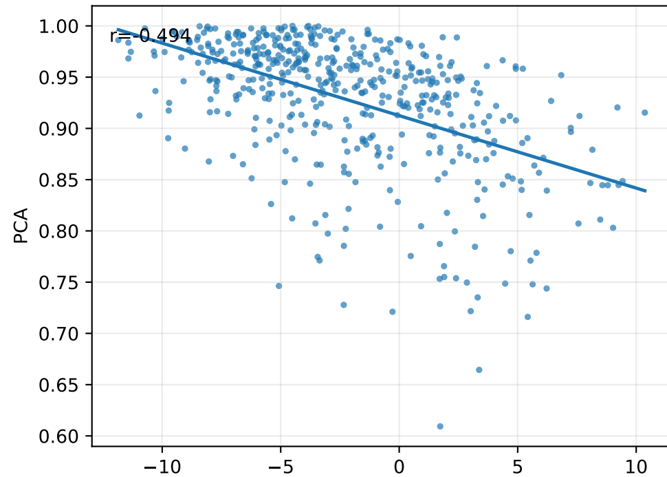
Semantic Similarity
