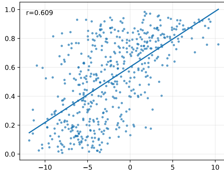
Levenshtein Distance
