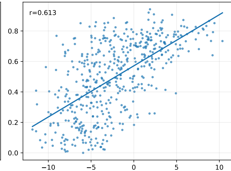
Jaccard Distance
