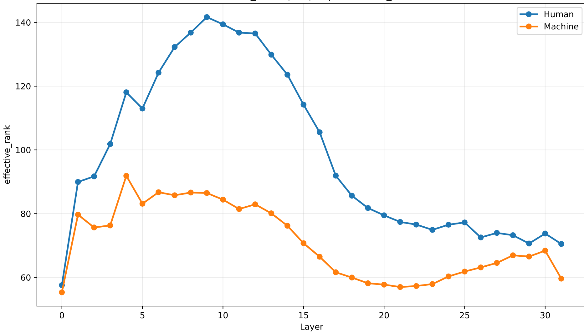
effective_rank by Layer | drlDomain_arxiv
