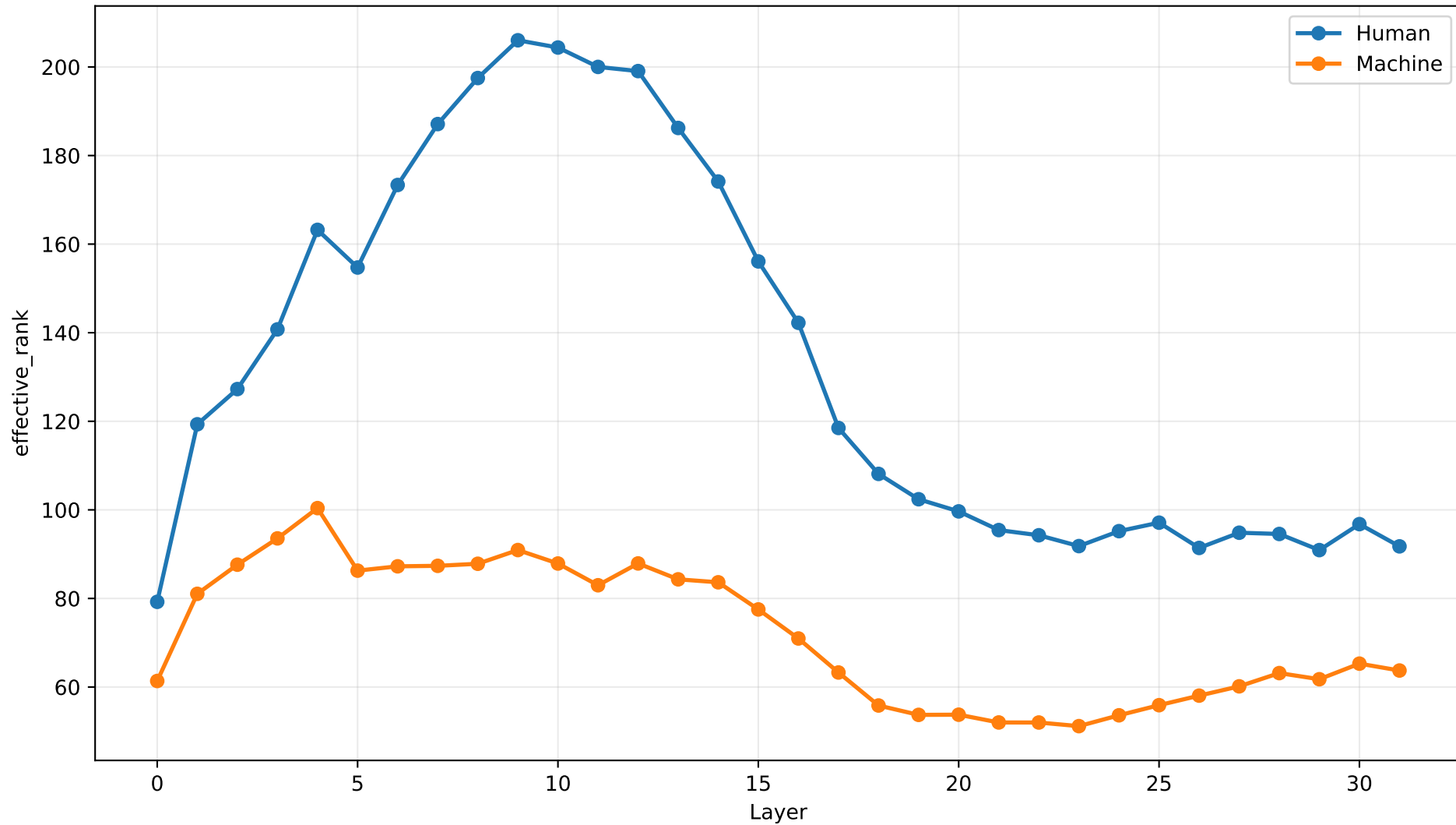
effective_rank by Layer | entropy_m4_arxiv
