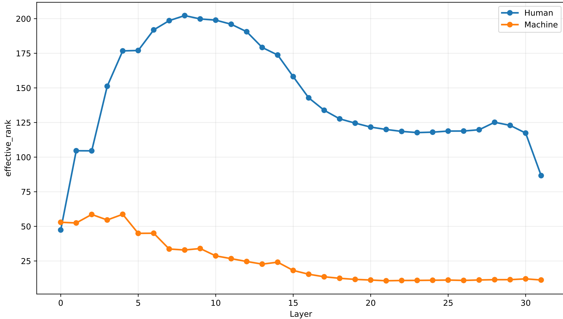
effective_rank by Layer | entropy_m4_peerread
