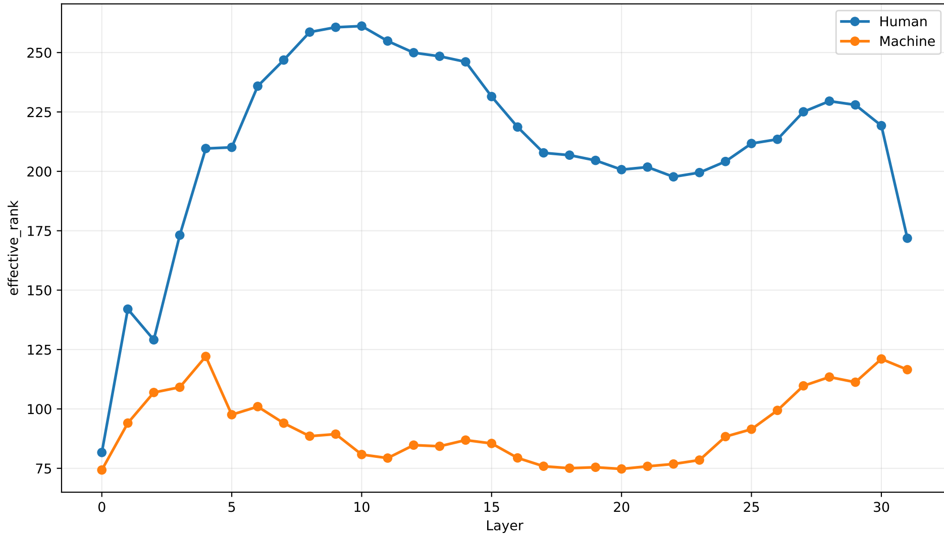
effective_rank by Layer | entropy_m4_wikipedia
