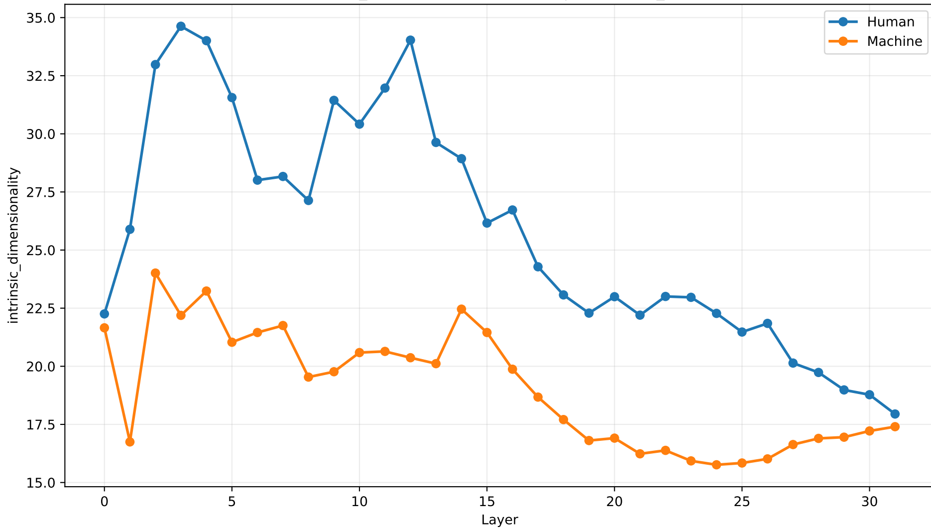
intrinsic_dimensionality by Layer | drlDomain_arxiv
