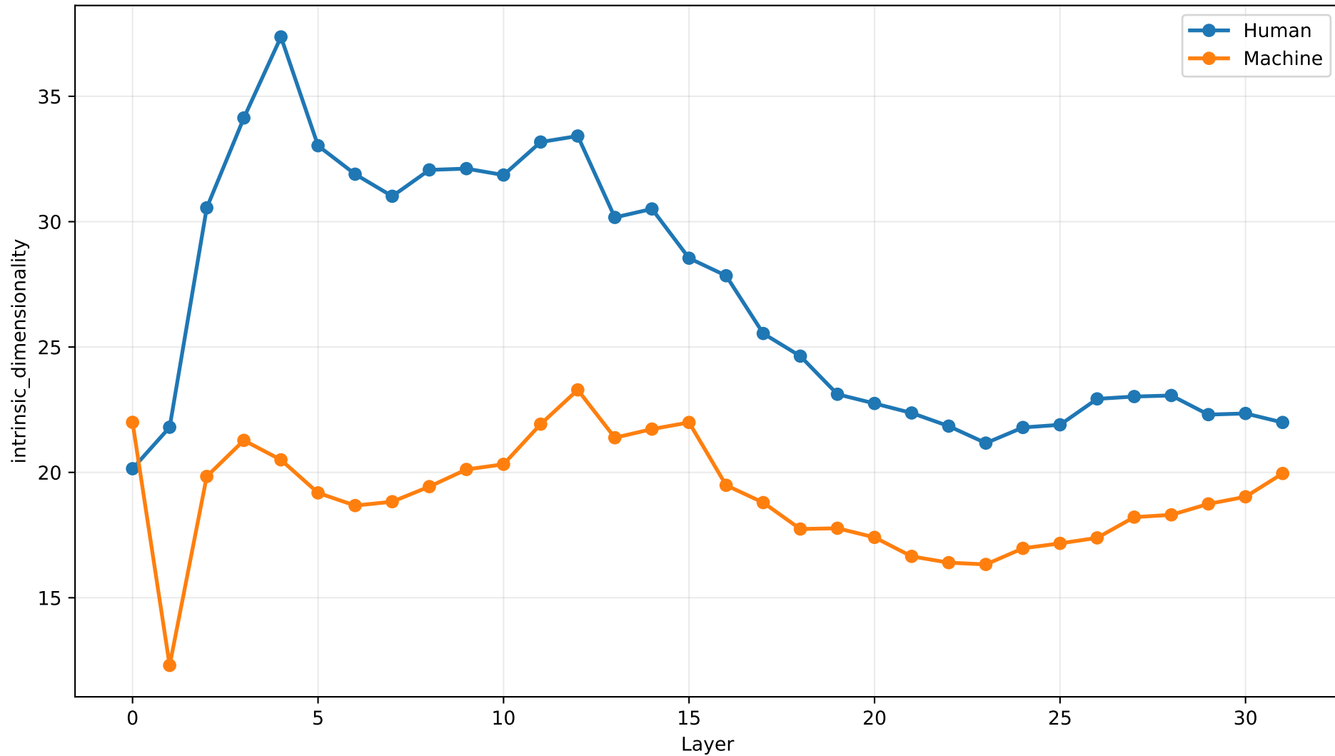
intrinsic_dimensionality by Layer | entropy_m4_arxiv
