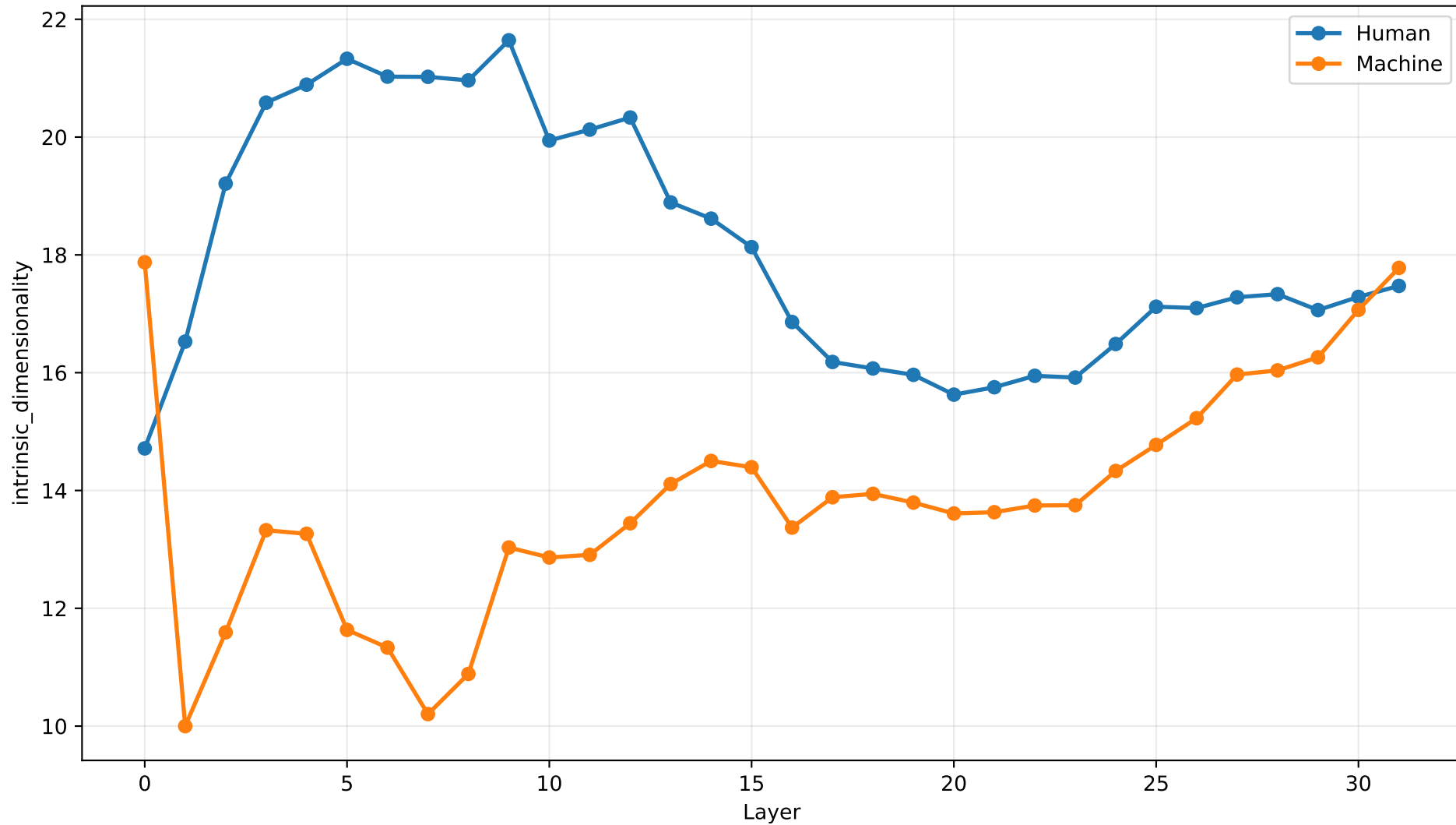
intrinsic_dimensionality by Layer | entropy_m4_peerread
