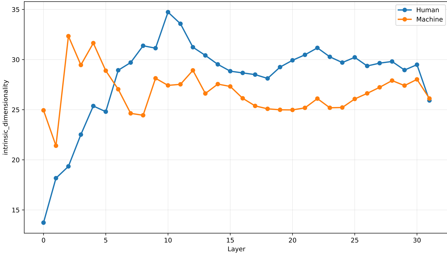
intrinsic_dimensionality by Layer | entropy_m4_reddit
