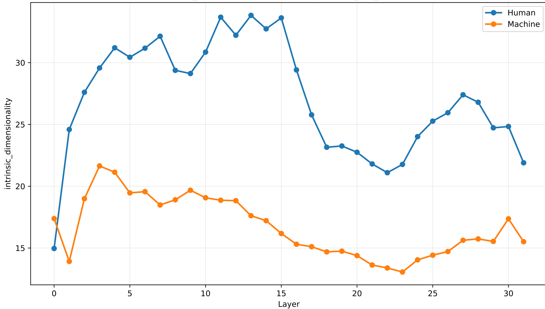
intrinsic_dimensionality by Layer | entropy_m4_wikipedia
