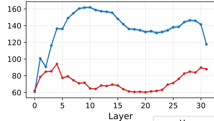
Effective Rank
