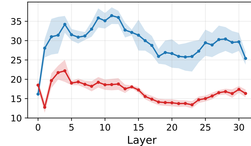
Intrinsic Dimensionality
