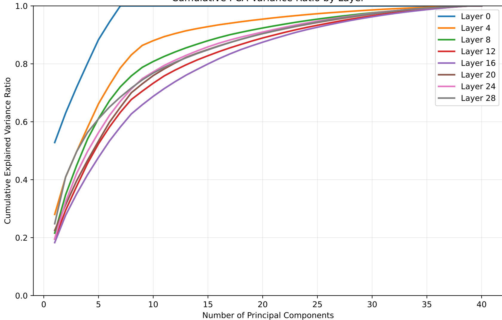
Cumulative PCA Variance Ratio by Layer
