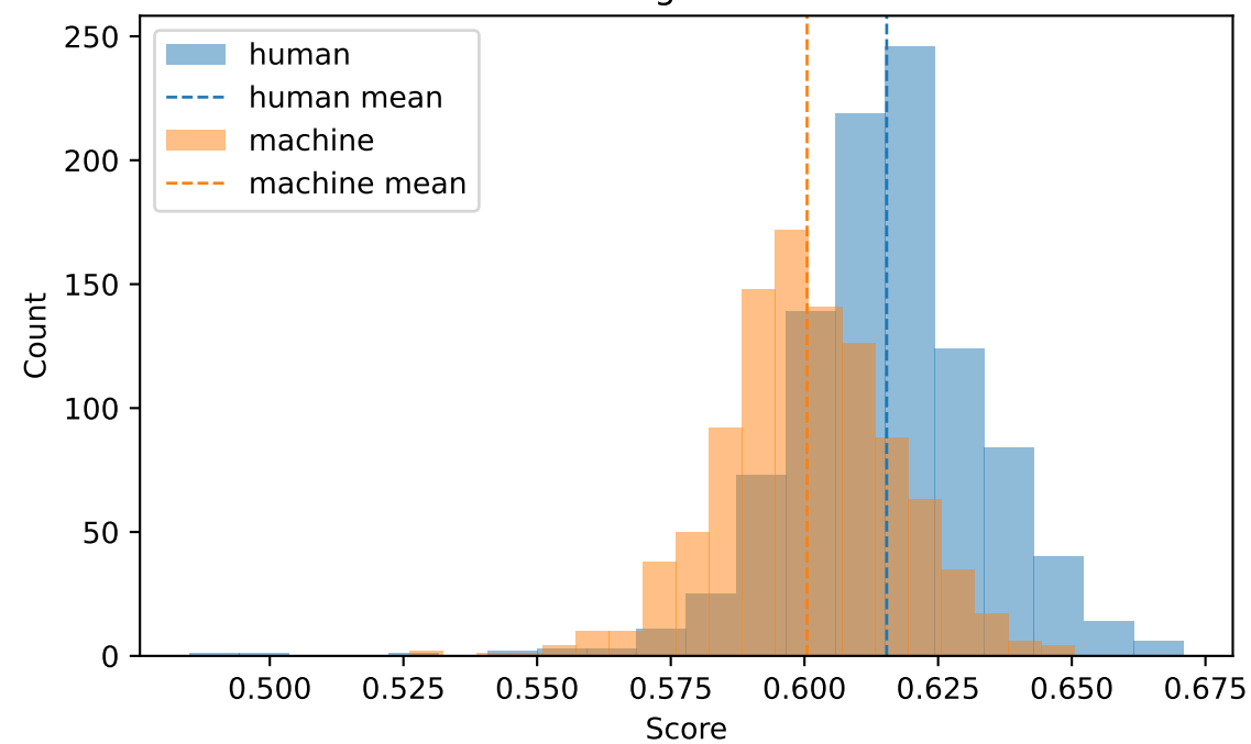
Length Std
