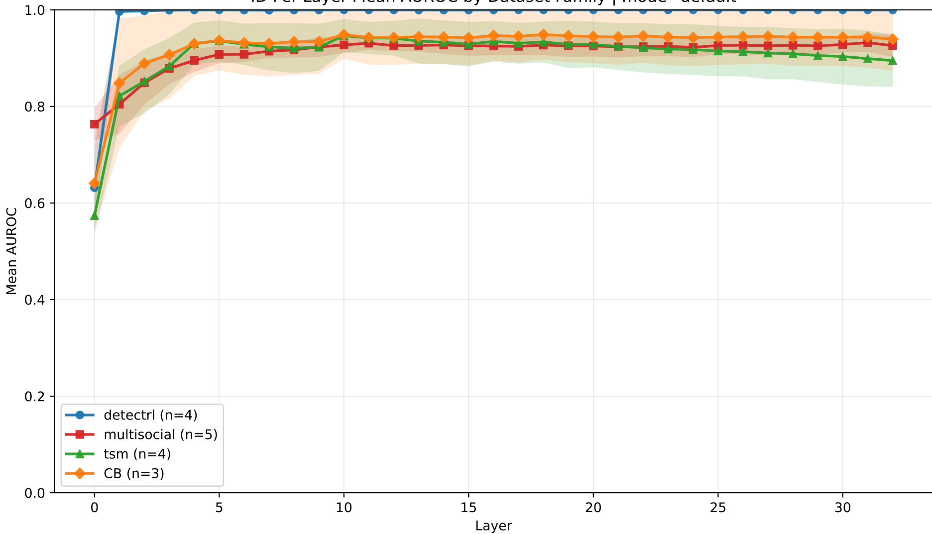
ID Per-Layer Mean AUROC by Dataset Family | mode=default
