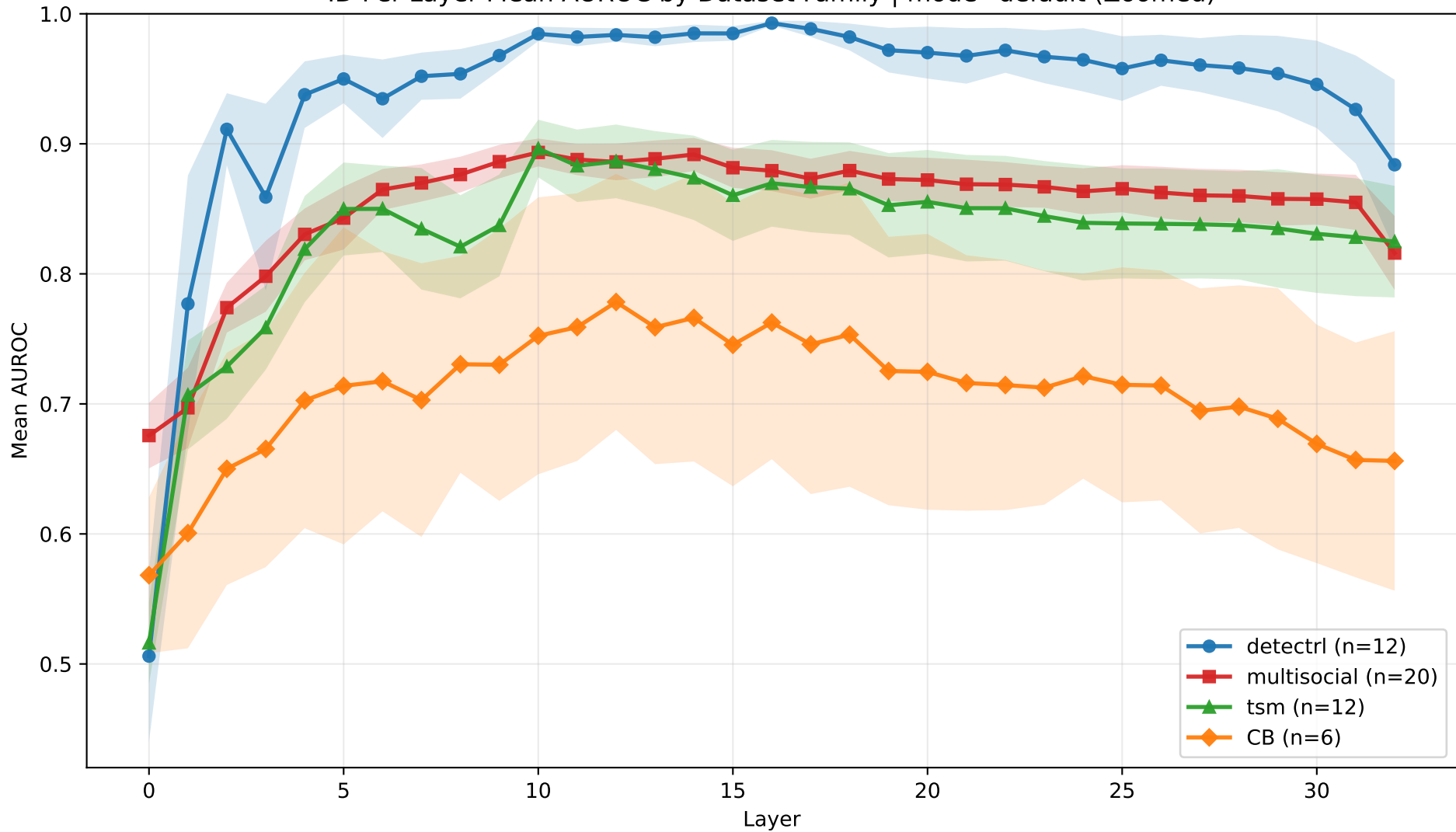
ID Per-Layer Mean AUROC by Dataset Family | mode=default (Zoomed)
