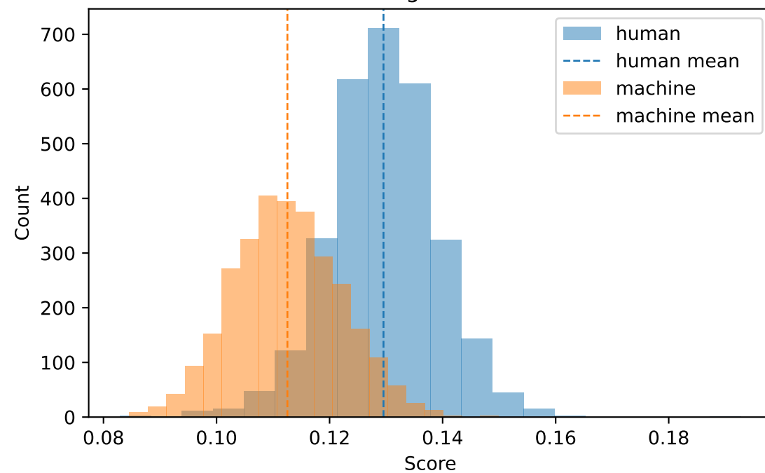
Magnitude Std
