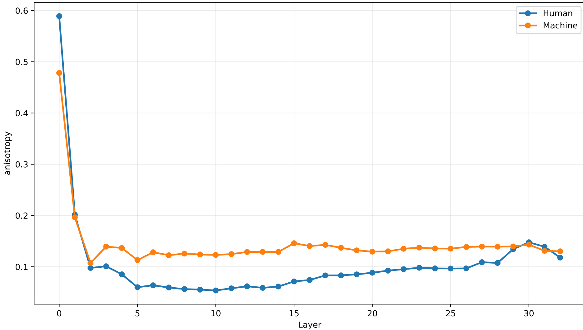
anisotropy by Layer | drlDomain_arxiv
