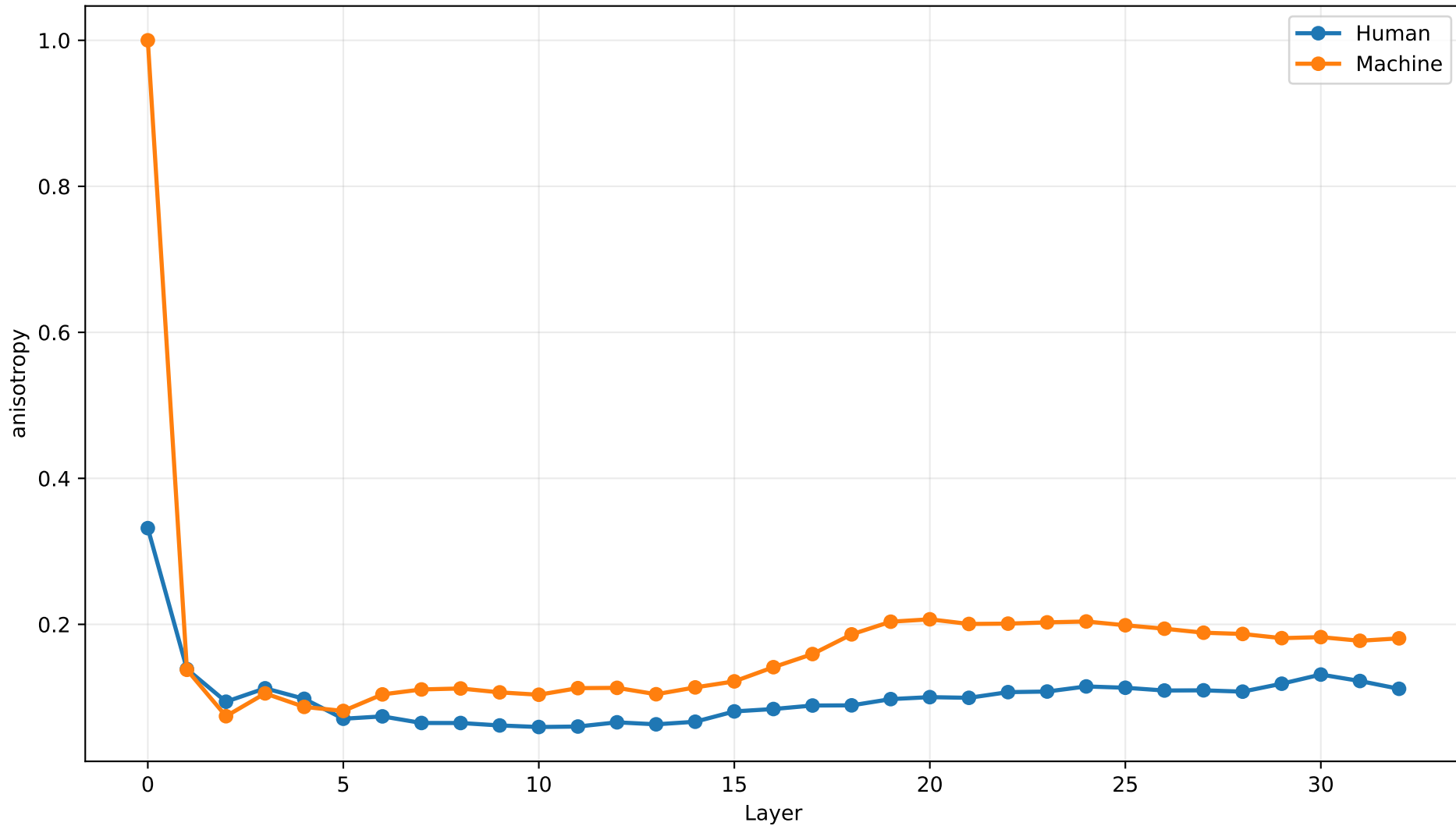
anisotropy by Layer | entropy_m4_arxiv
