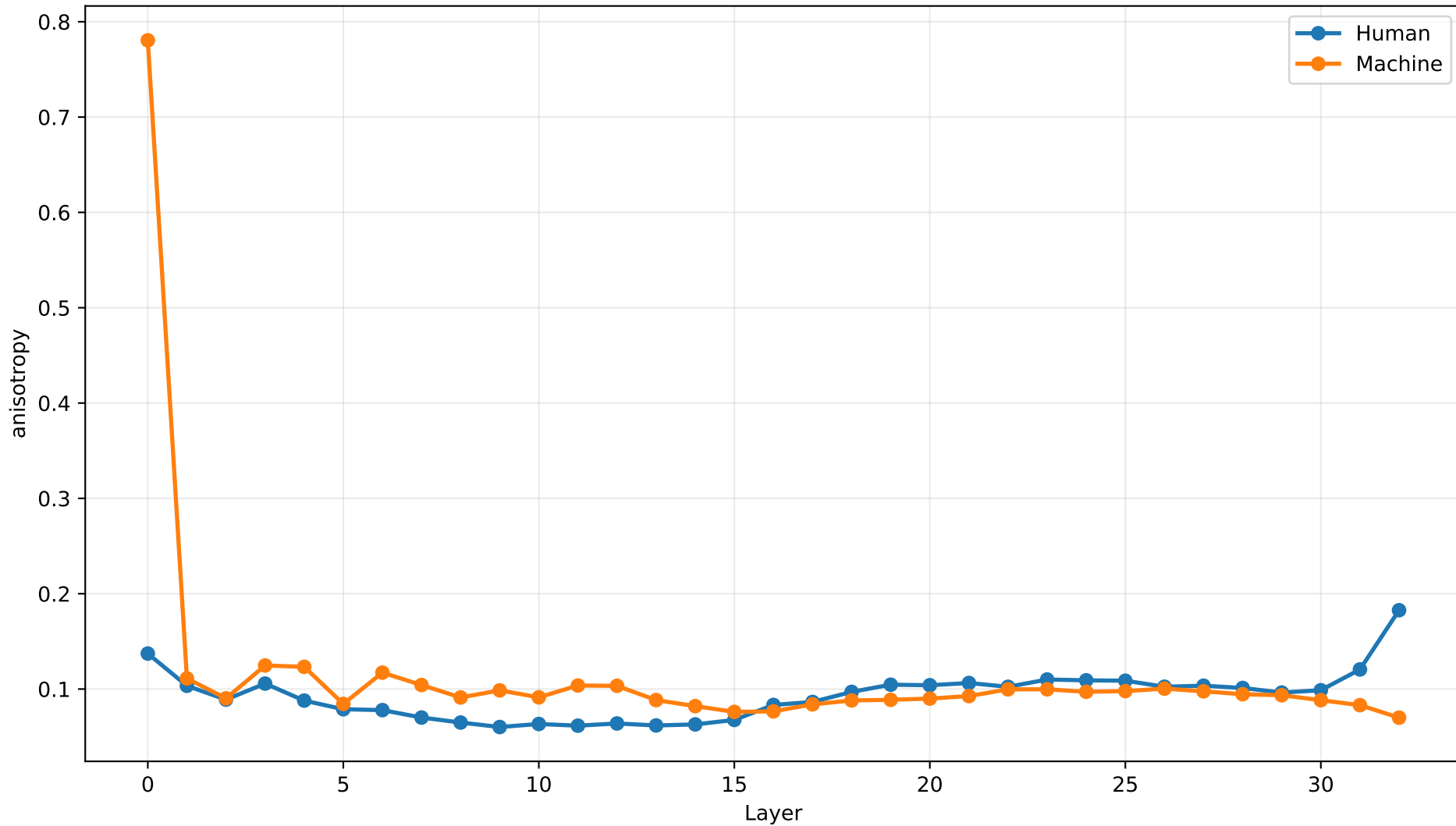
anisotropy by Layer | entropy_m4_reddit
