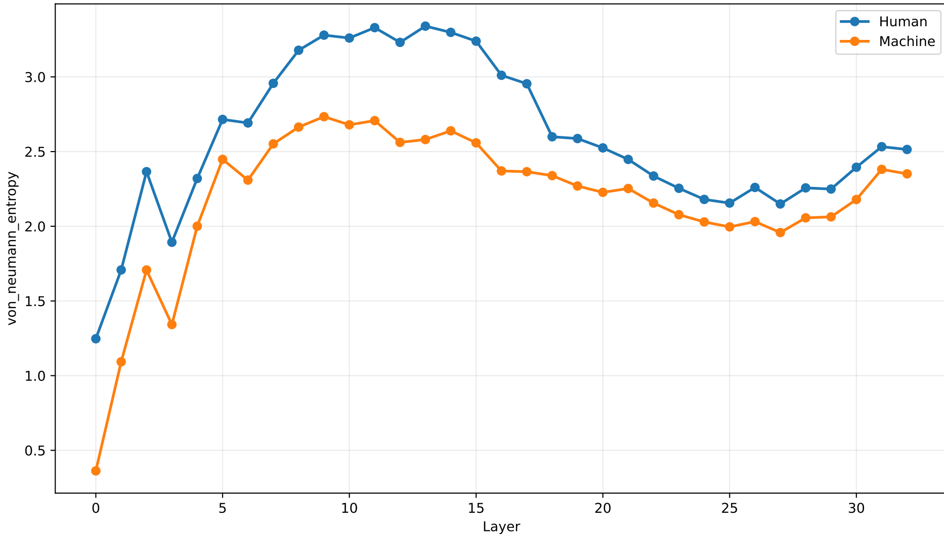
von_neumann_entropy by Layer | drlDomain_xsum
