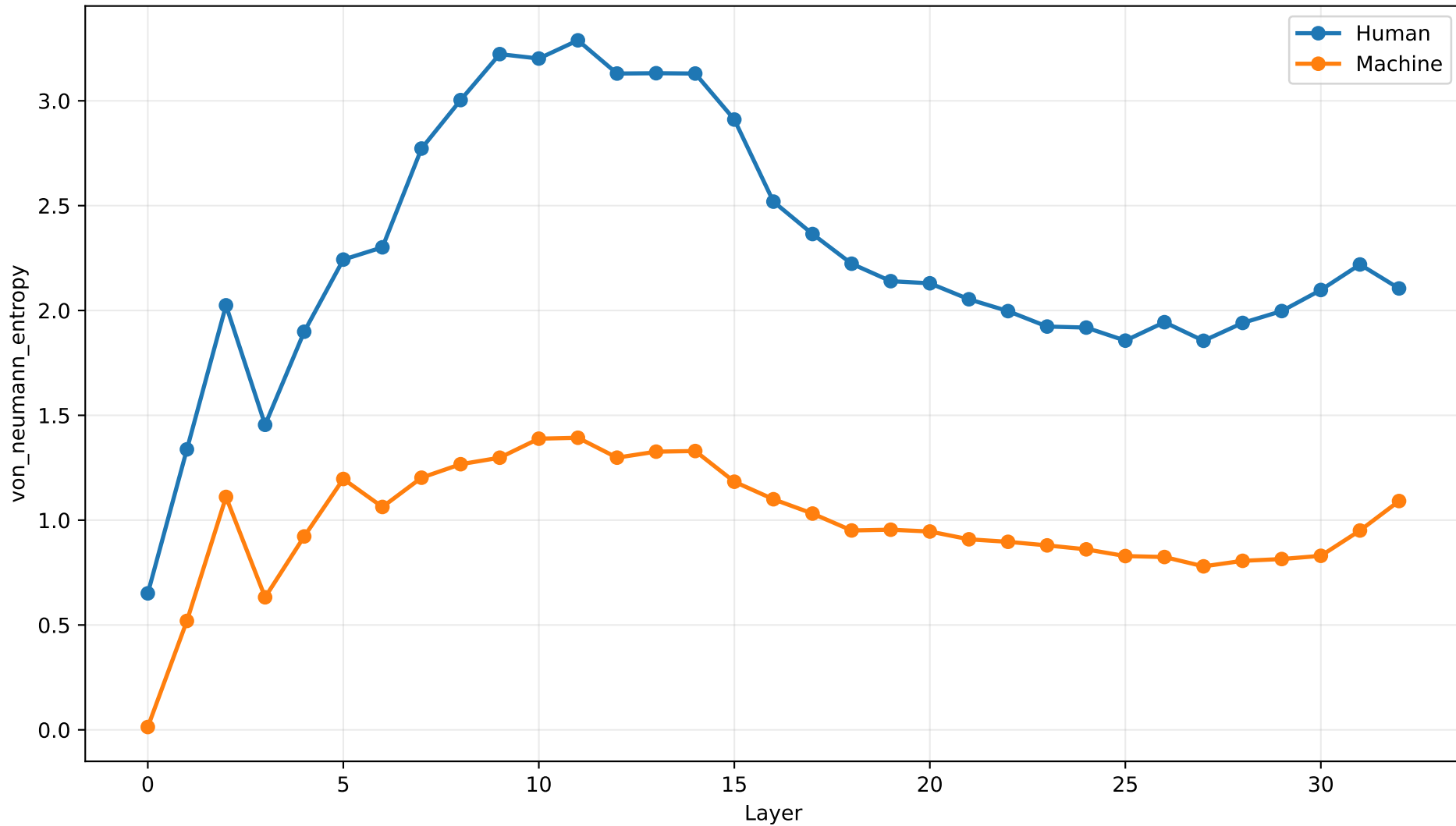
von_neumann_entropy by Layer | entropy_m4_arxiv
