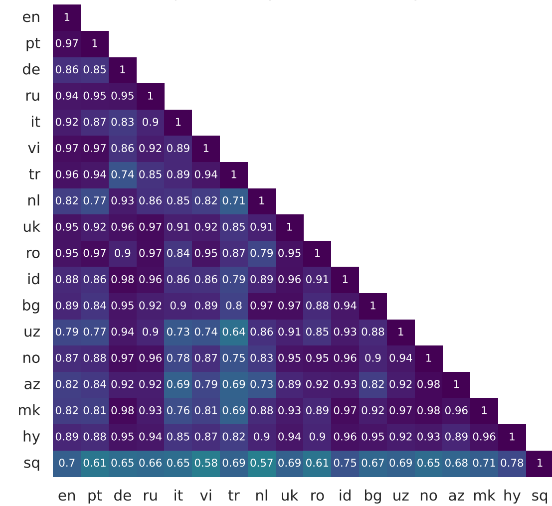
(b) Topic Similarity (Cosine Similarity [-1,1])
