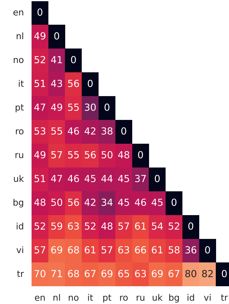
(b) lang2vec (Syntactic Distance [0,1])
