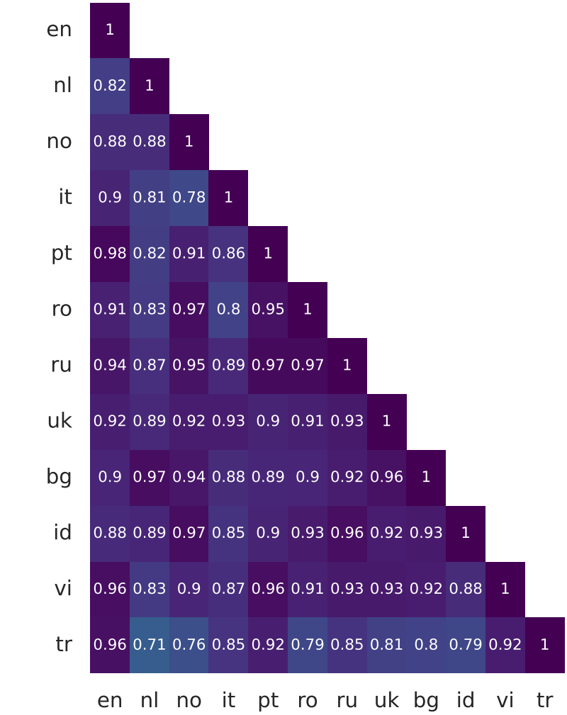
(c) Topic Similarity (Cosine Similarity [-1,1])
