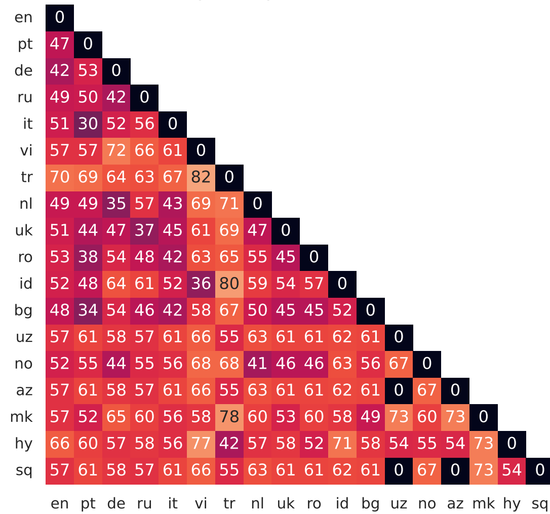
(a) lang2vec (Syntactic Distance [0,1])
