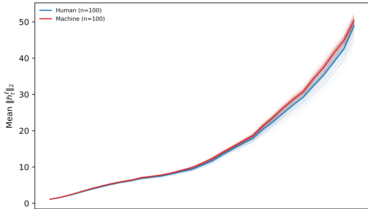
l8b, drlXDomainLen_wiki_500_tokens: across-layer depth profile (raw states, layers 1..L-1, first 10 tokens left out); lines: texts, solid: group mean with 95% CI; bottom: AUC P(M > H)
