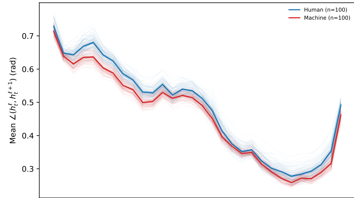
l8b, drlXDomainLen_wiki_500_tokens: across-layer depth profile (raw states, layers 1..L-1, first 10 tokens left out); lines: texts, solid: group mean with 95% CI; bottom: AUC P(M > H)
