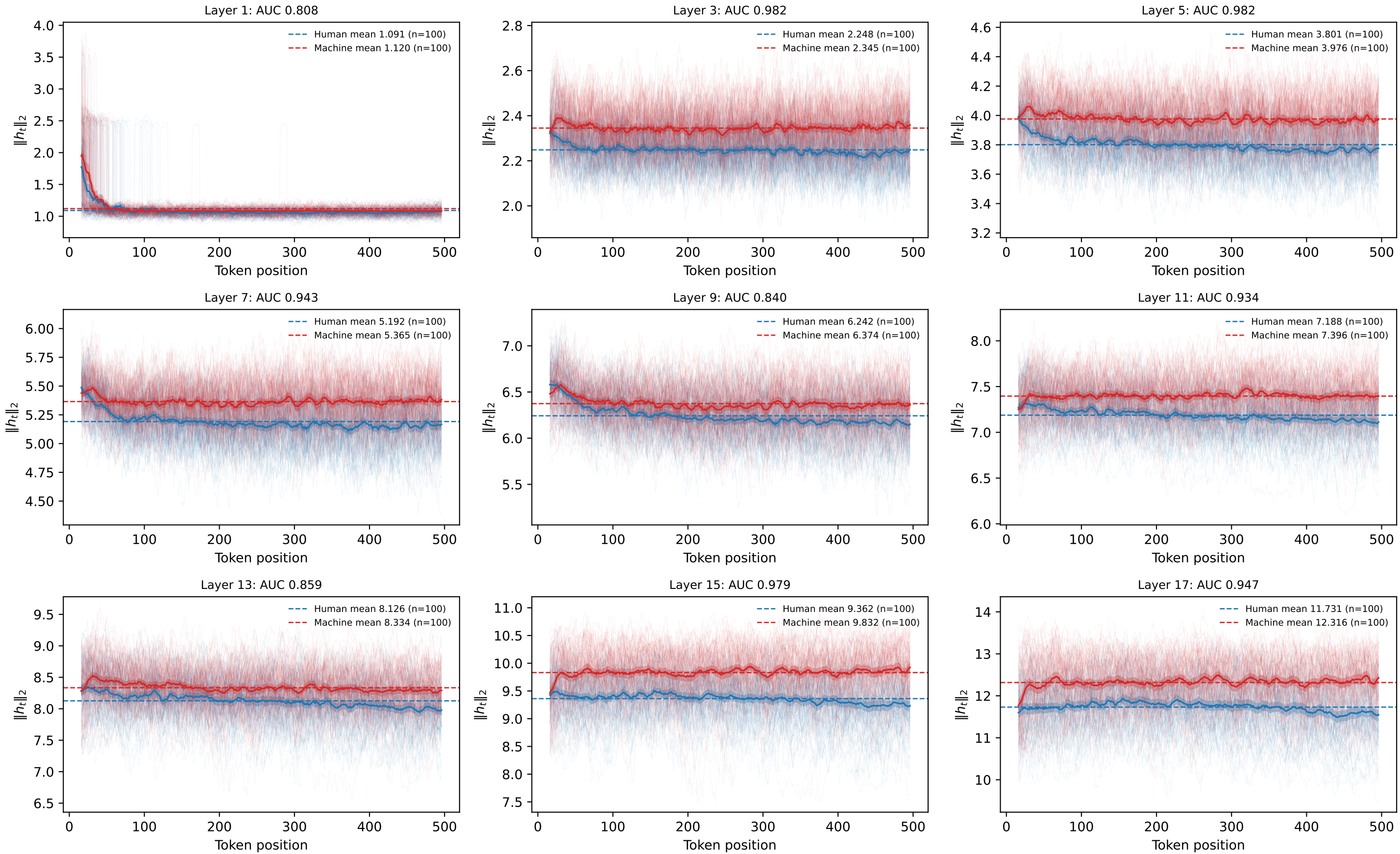
l8b, drlXDomainLen_wiki_500_tokens: within-layer norm per token (raw states, first 10 tokens left out); lines: rolling mean over 10 tokens, solid: group mean with 95% CI
