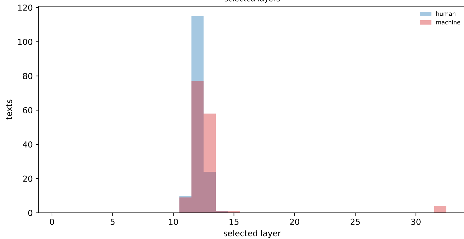
selected layers
