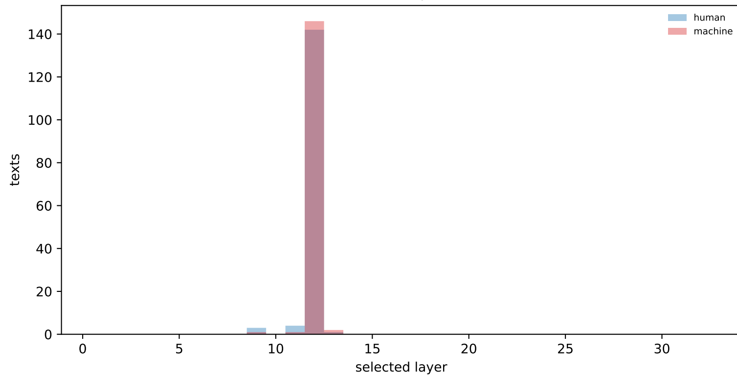
selected layers
