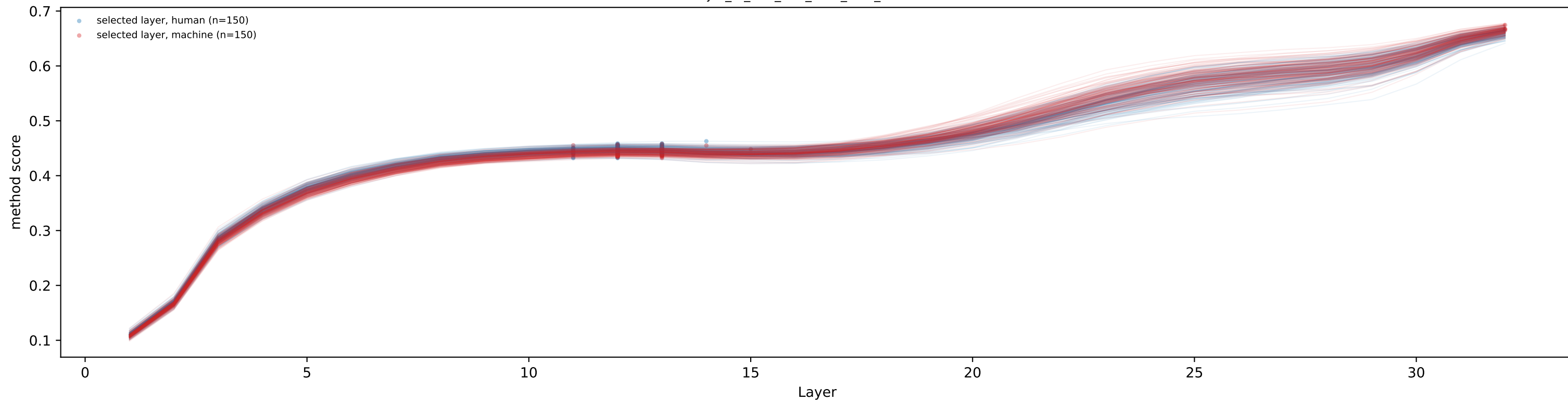
selected layers
