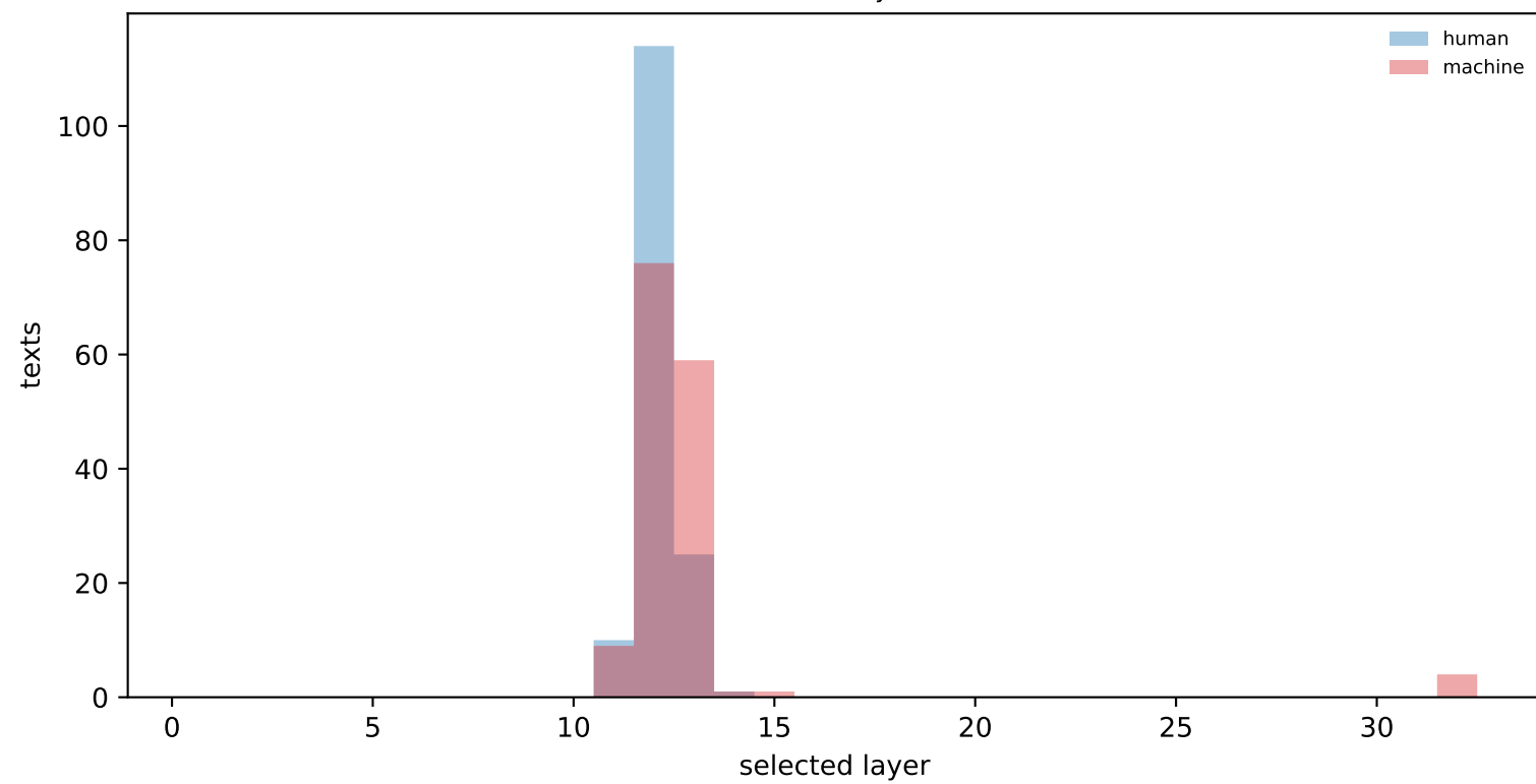
selected layers
