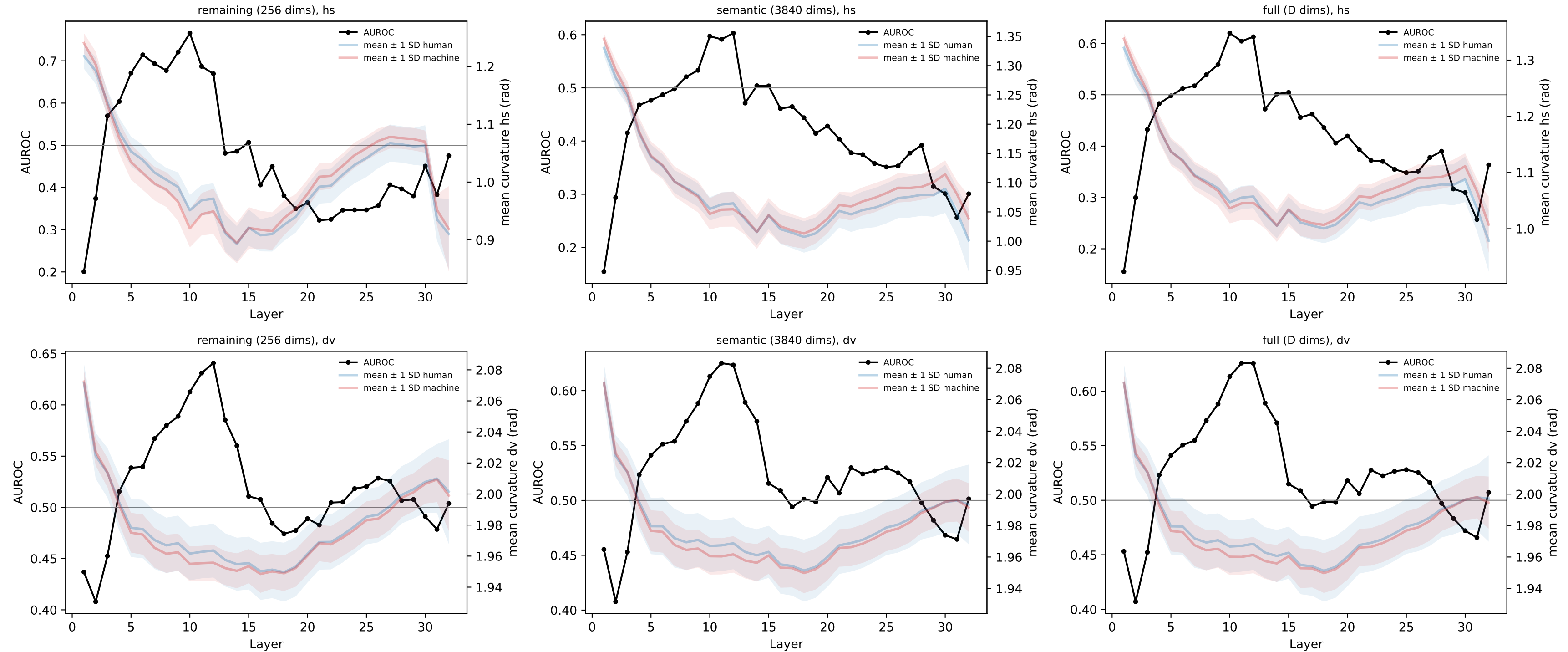
l8b, drlXAttacks_character_deletion: curvature per subspace of W_U
