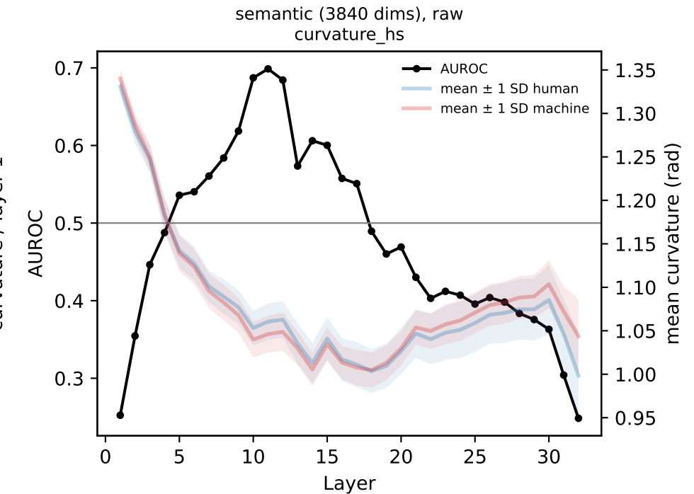
l8b, drlXAttacks_decoder_paraphrasing: curvature per subspace of W_U
