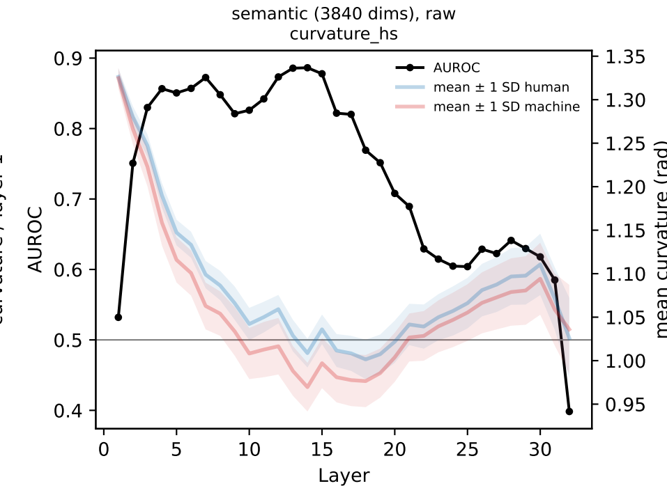
l8b, raidDomain_wiki: curvature per subspace of W_U
