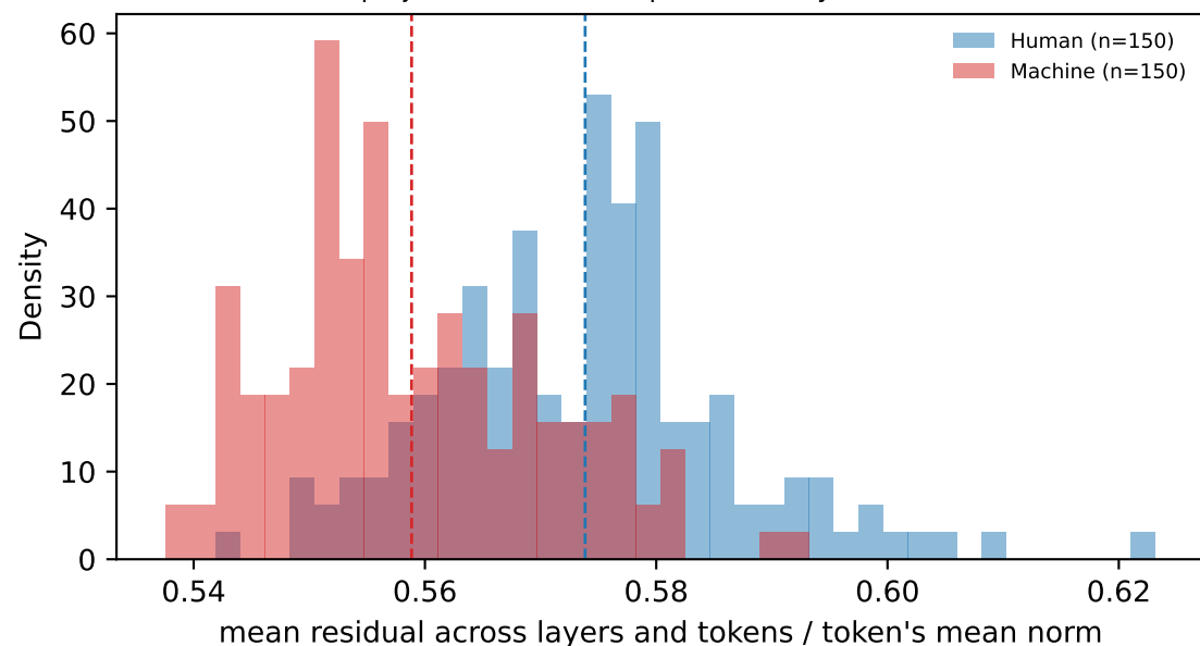
rel_error, projected on mean of previous 3 layers: AUROC=0.814
