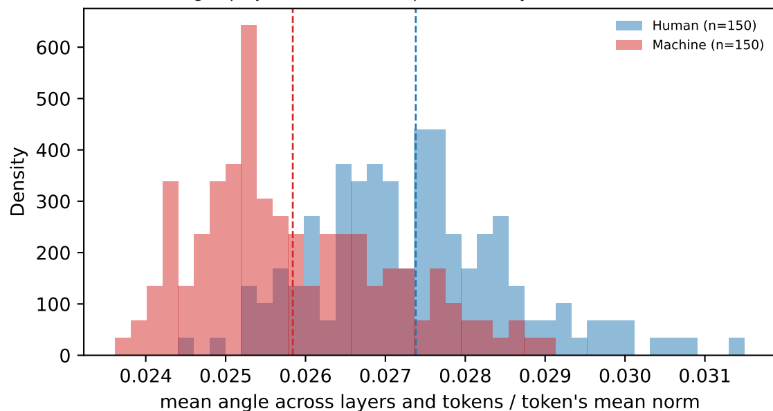
residual, projected on mean of previous 3 layers: AUROC=0.190
