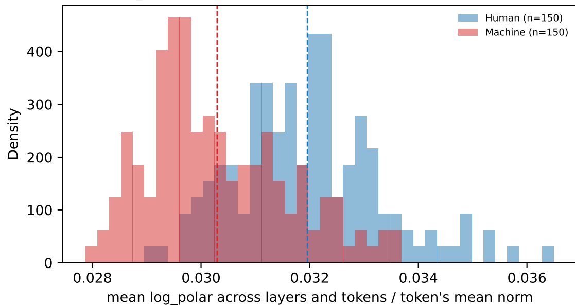
log_polar, projected on mean of previous 3 layers: AUROC=0.816
