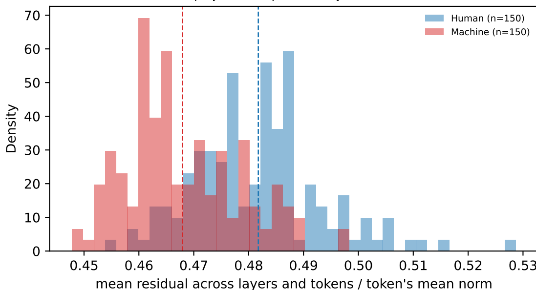
rel_error, projected on previous layer: AUROC=0.806
