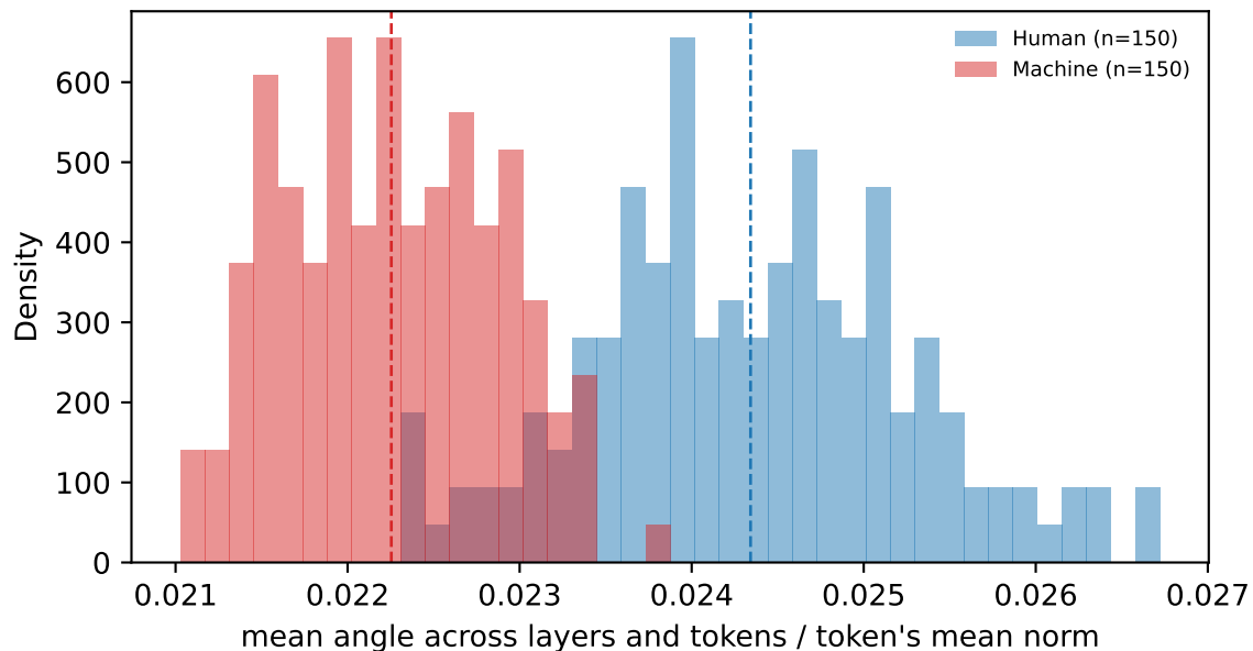
l8b, drlXDomain_academic: projection across layers, divided by each token's mean norm
