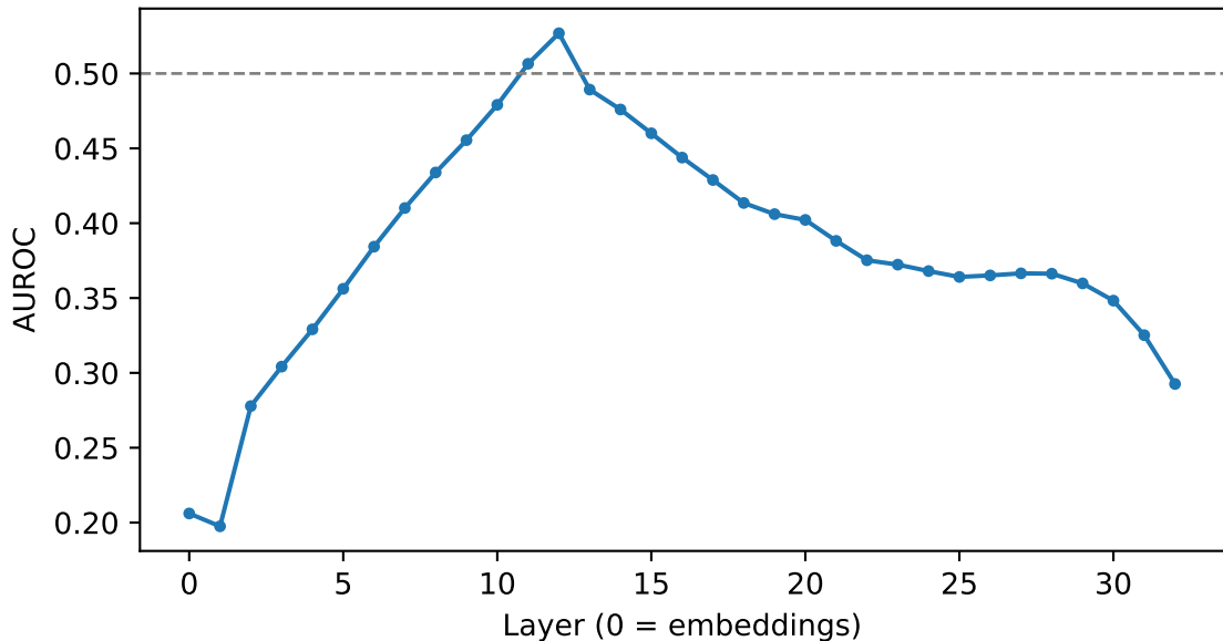
Log-det novelty ( \lambda=1.0 ): l8b, drlXAttacks_character_deletion
