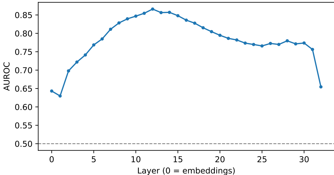
Log-det novelty ( \lambda=1.0 ): l8b, raidDomain_wiki
