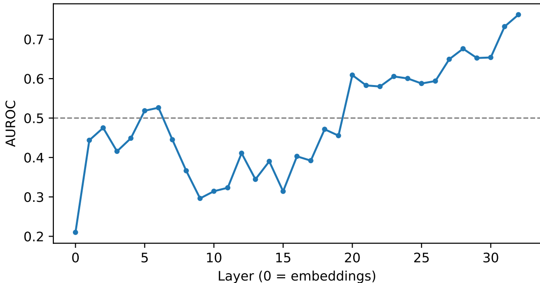
Instruct vs. base divergence: l8b, drlXAttacks_character_deletion
