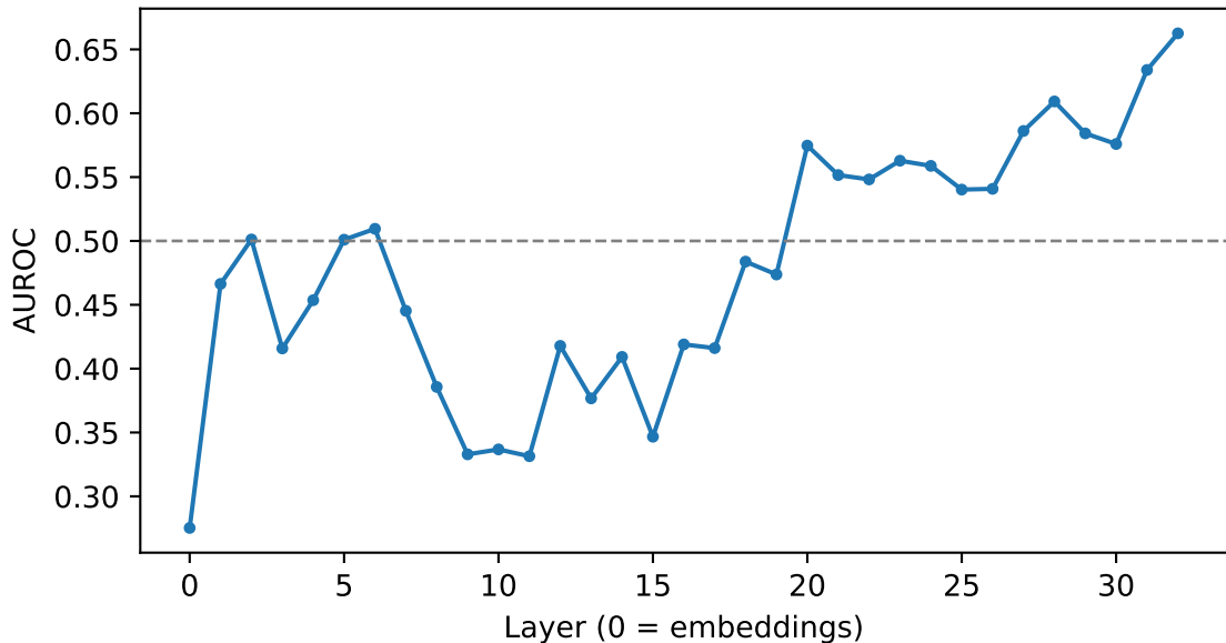
Instruct vs. base divergence: l8b, drlXAttacks_decoder_paraphrasing
