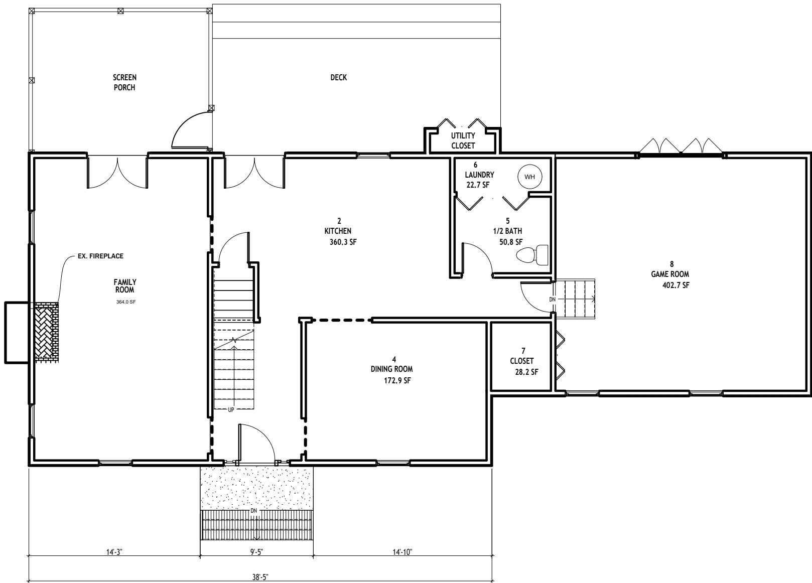
1ST LEVEL PROPOSED FLOOR PLAN
