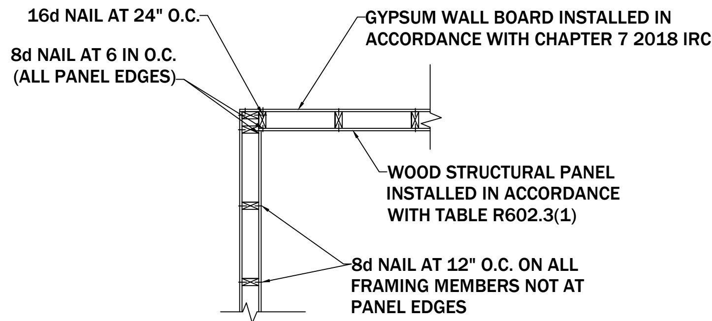
21 INSIDE CORNER DETAIL SCALE: NTS
