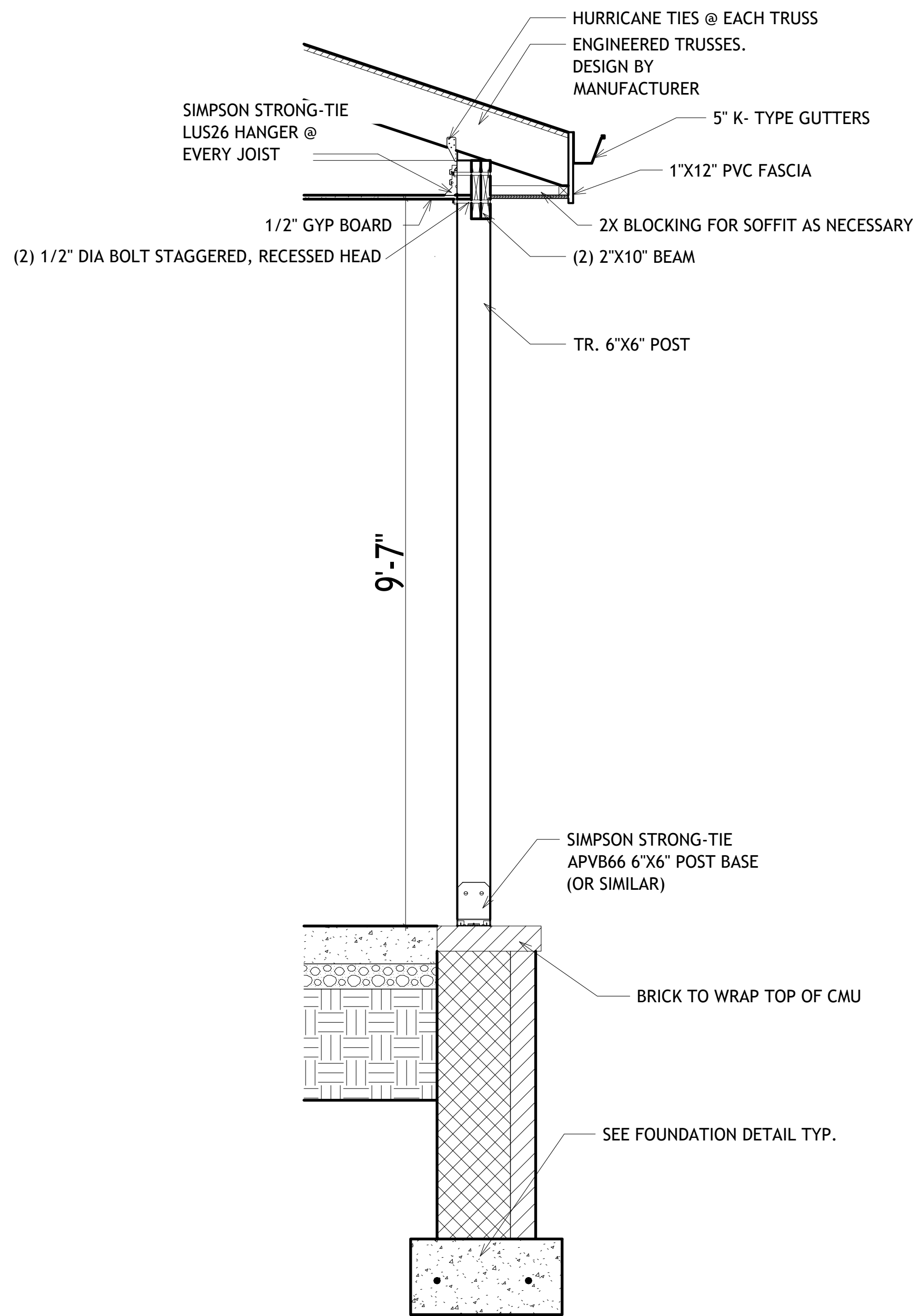
20 BACK PORCH POST ATTACHMENT AND ROOF DETAIL SCALE: 3/4"= 1'
