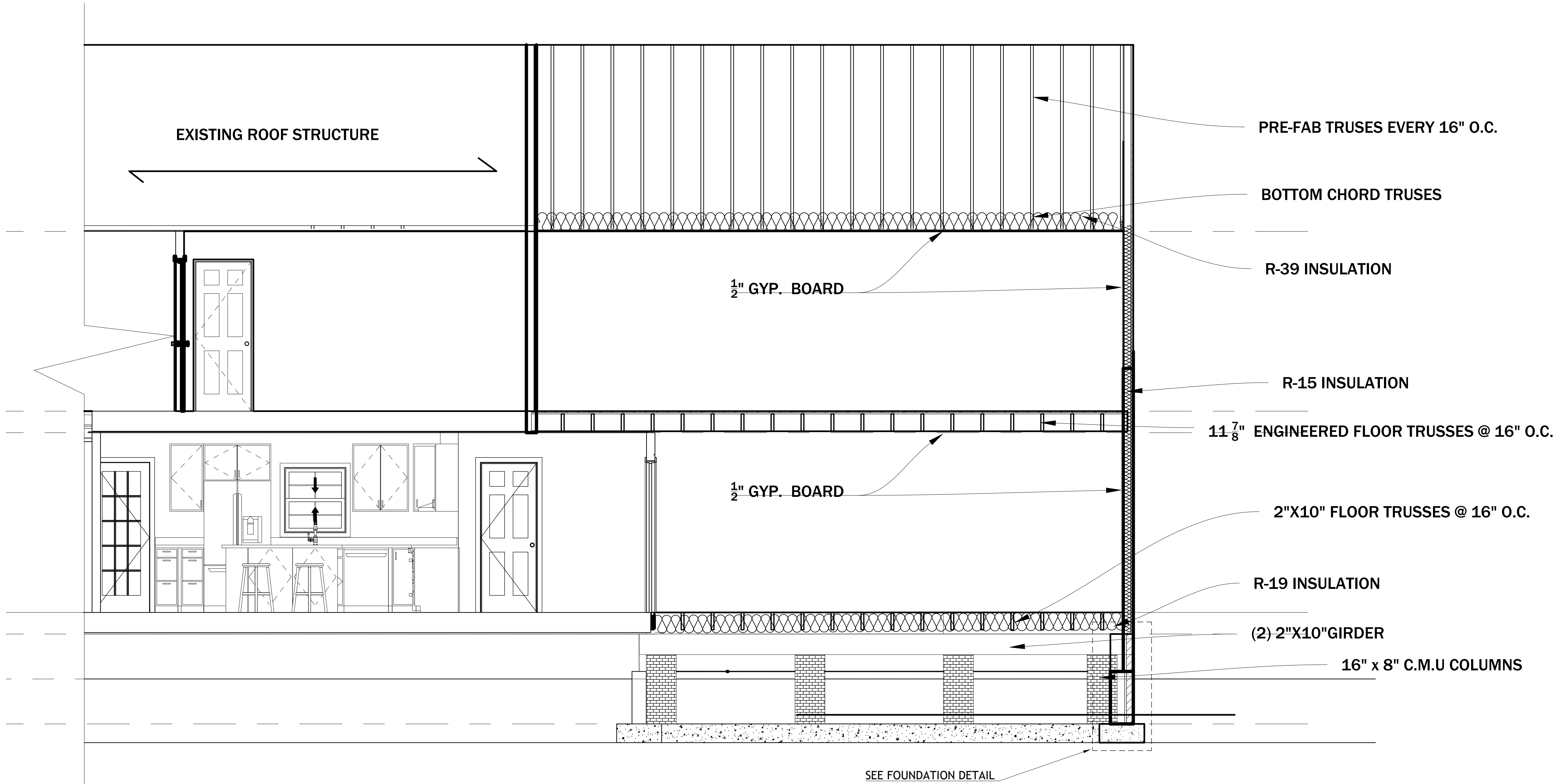
18 WALL SECTION
