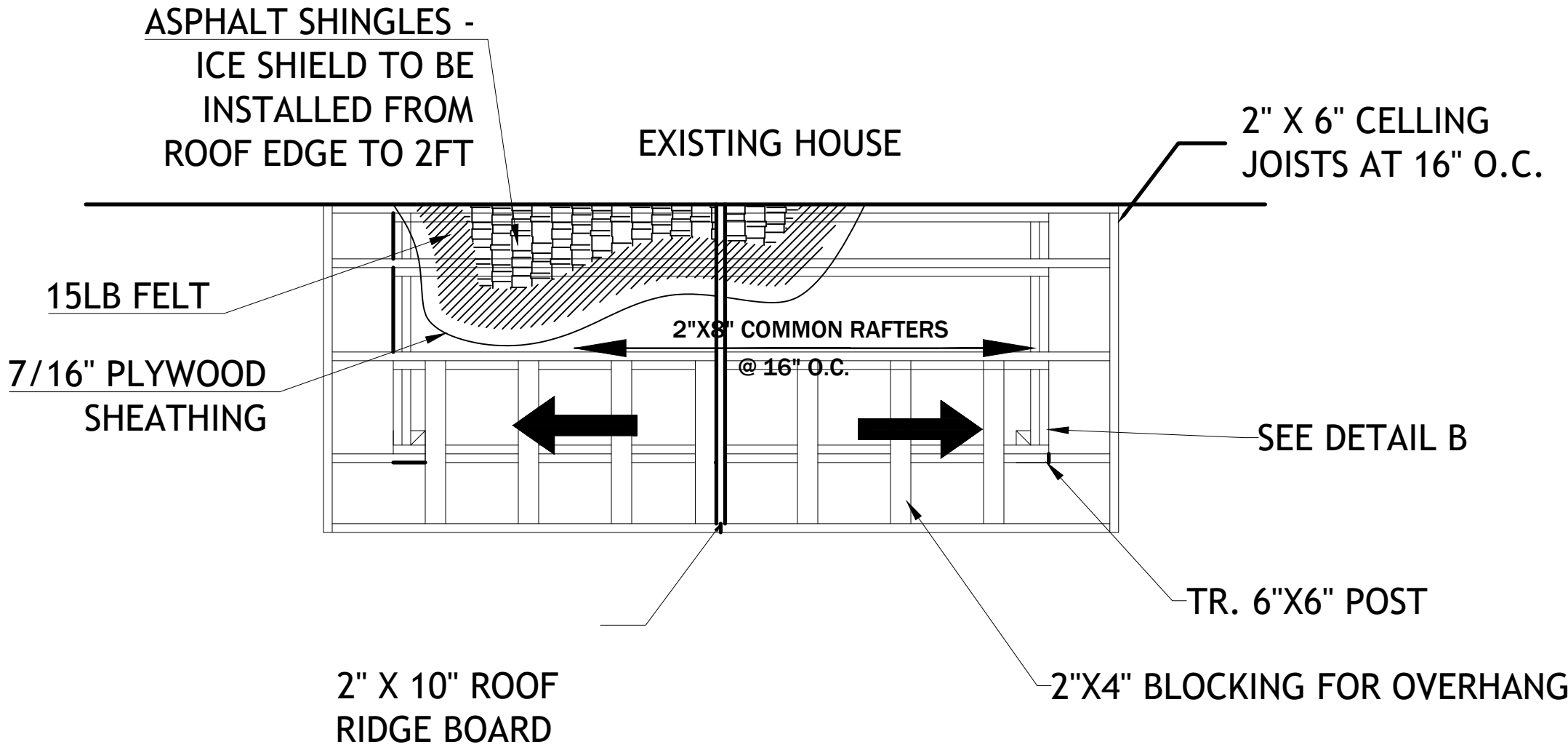
15 BACK PORCH ROOF PLAN SCALE: 3/8" = 1'-0"
