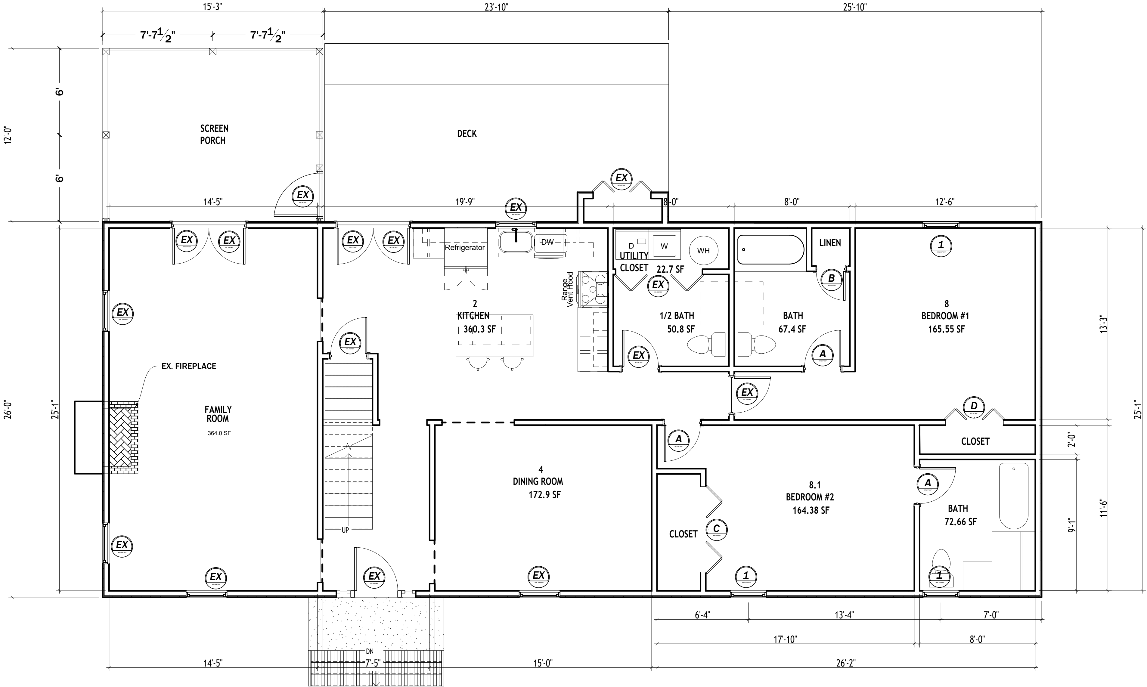
5 1ST LEVEL PROPOSED FLOOR PLAN
