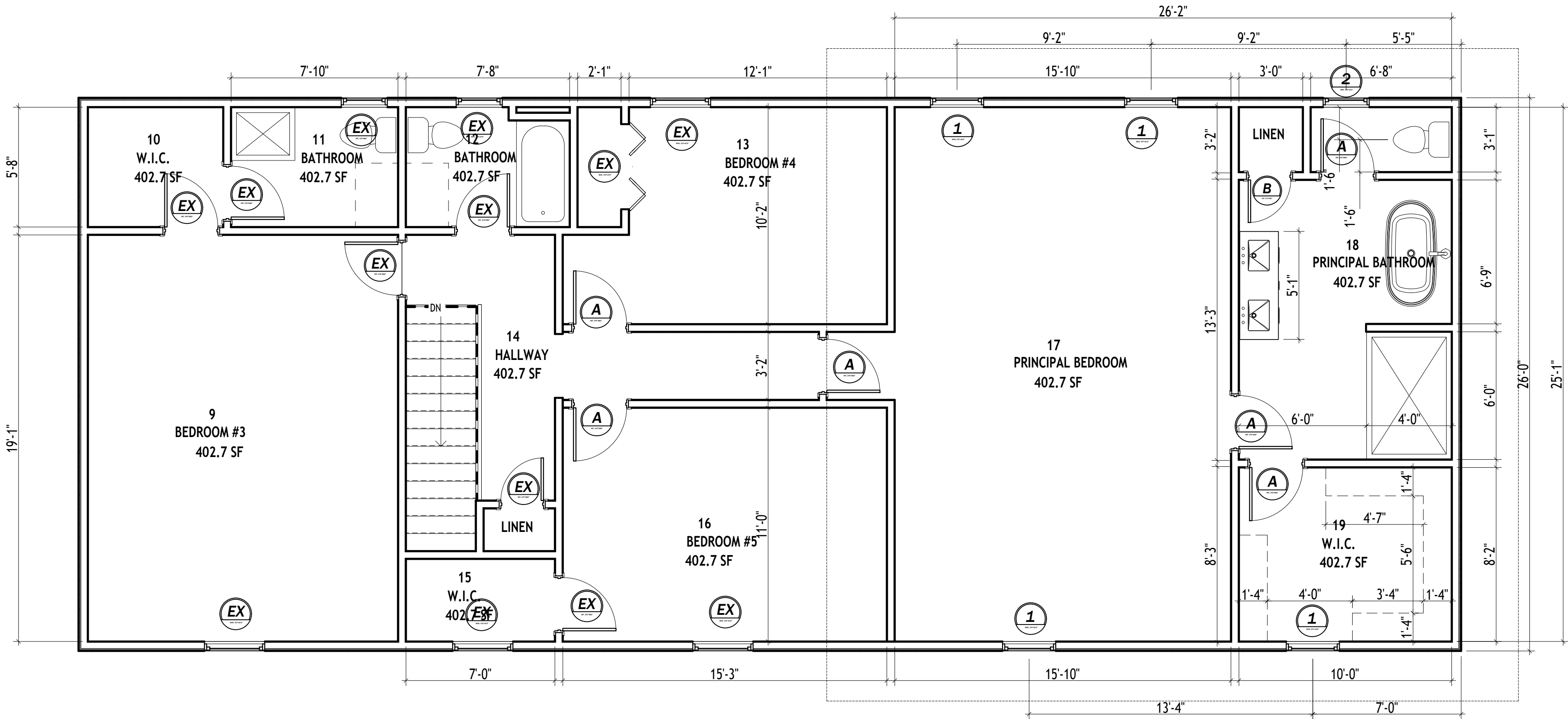
6 2ND LEVEL FLOOR PLAN SCALE: 1/4" = 1'
