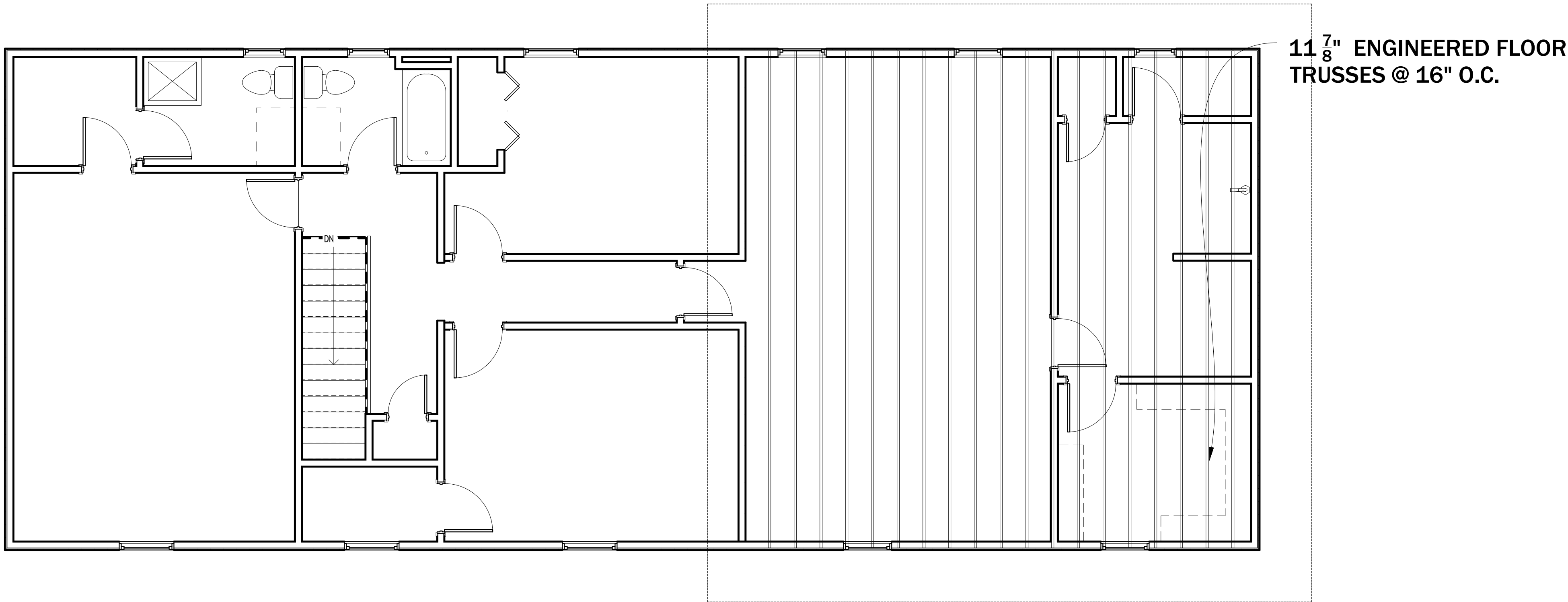
7 2ND LEVEL FLOOR FRAMING PLAN SCALE: 1/4" = 1'
