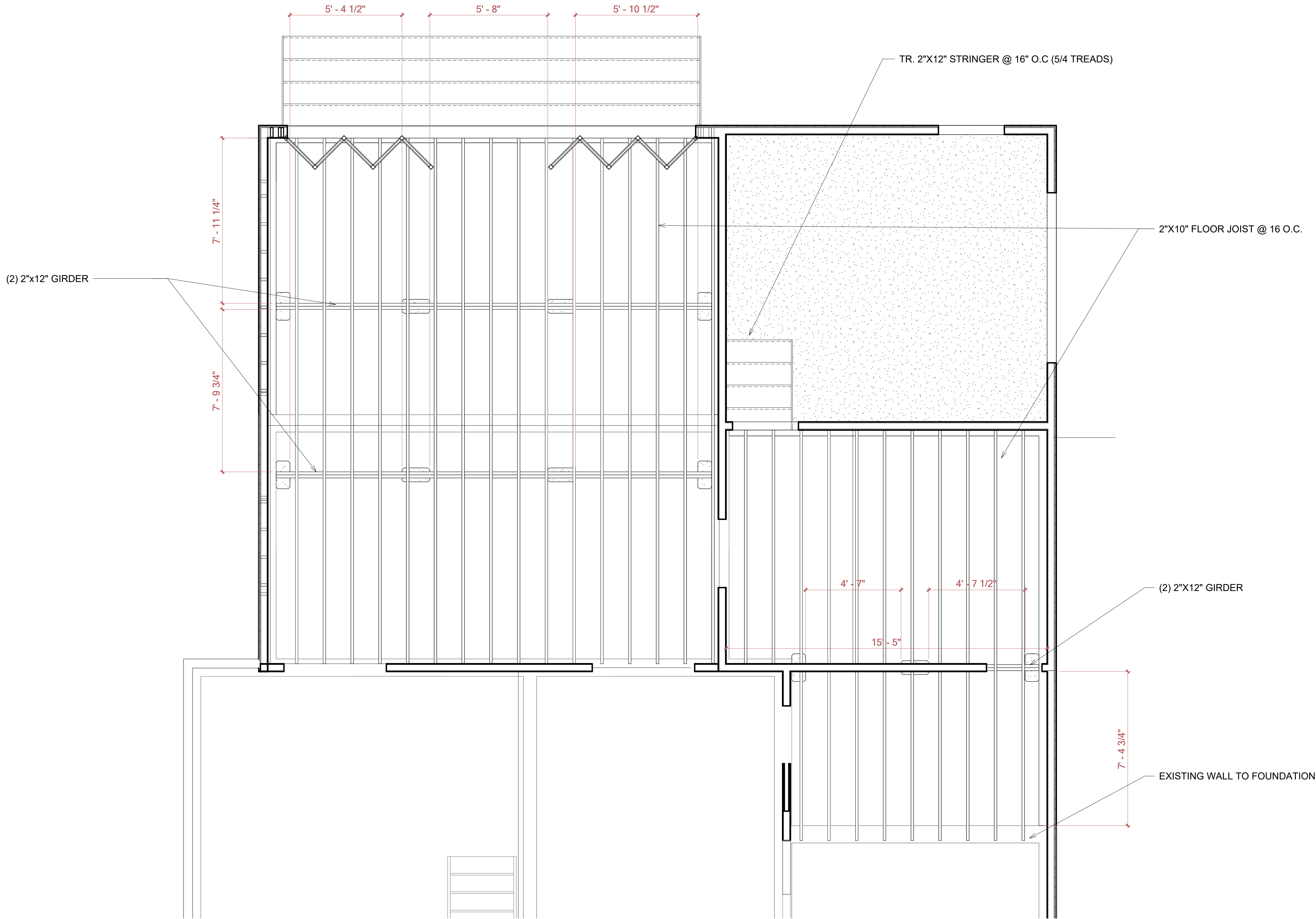
1 S.F.P - FLOOR FRAMING PLAN 3/8" = 1'-0"
