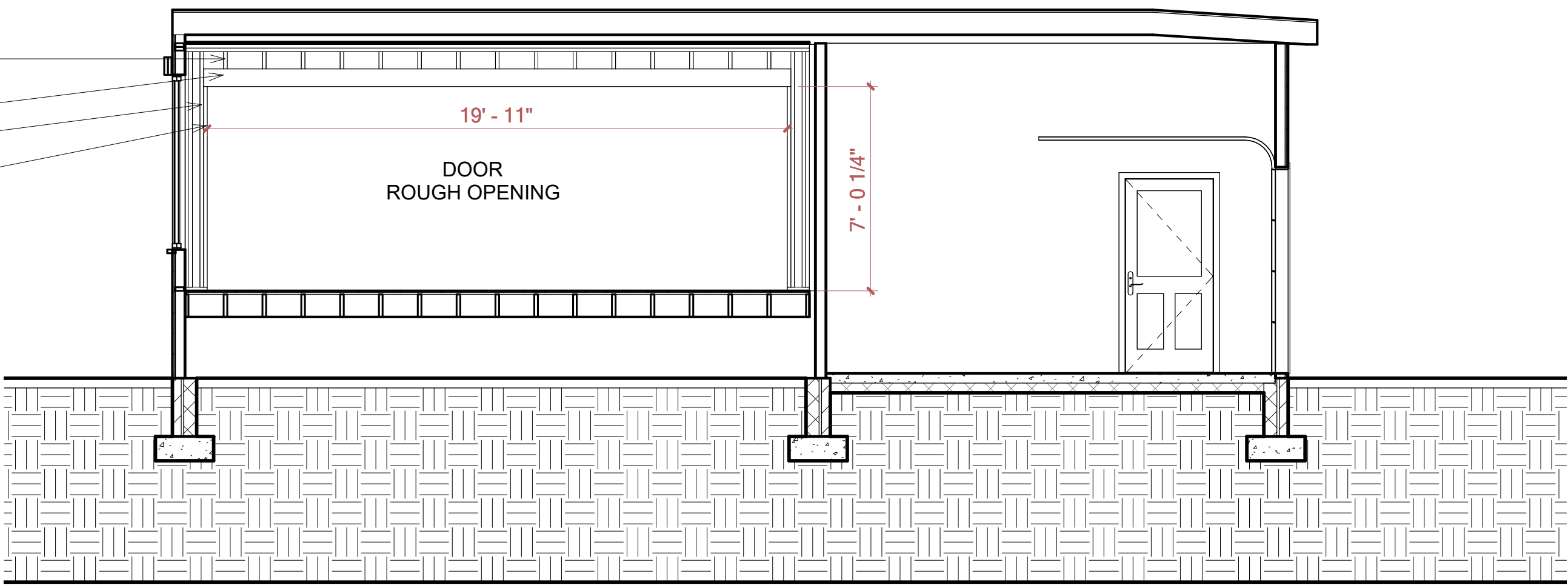
5 REAR WALL FRAMING DETAIL 1/4" = 1'-0"
