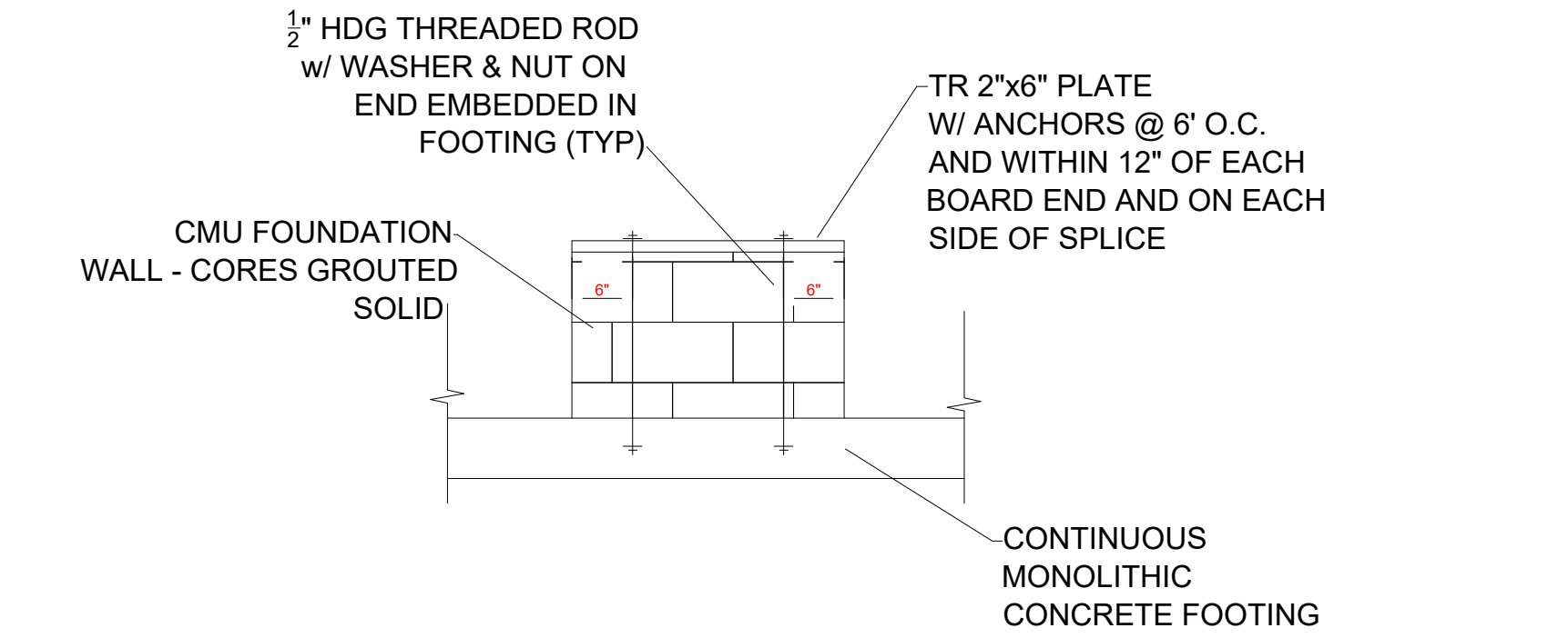
4 STEM WALL DETAIL 12" = 1'-0"
