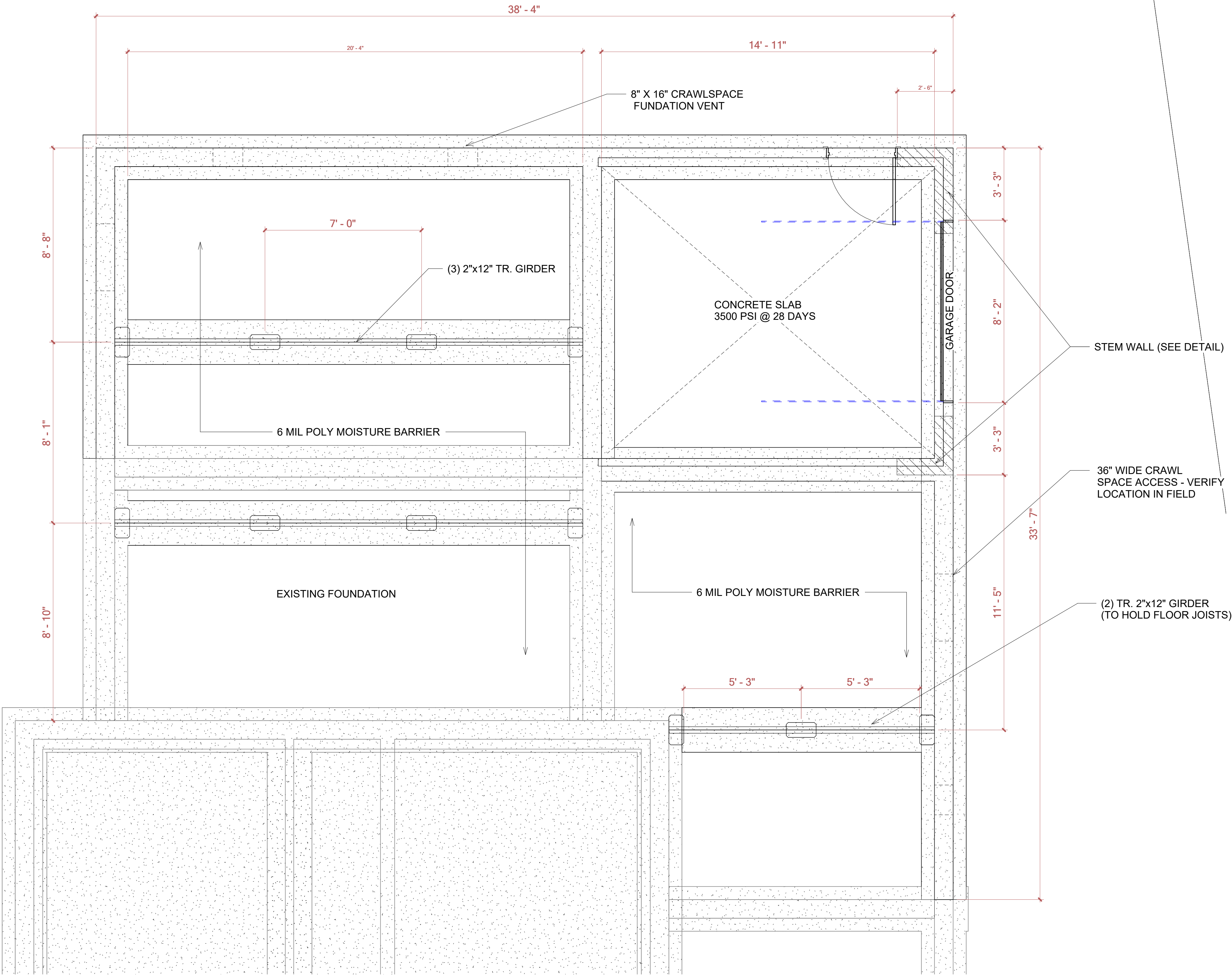
1 S.F.P. FOUNDATION PLAN 3/8" = 1'-0"
