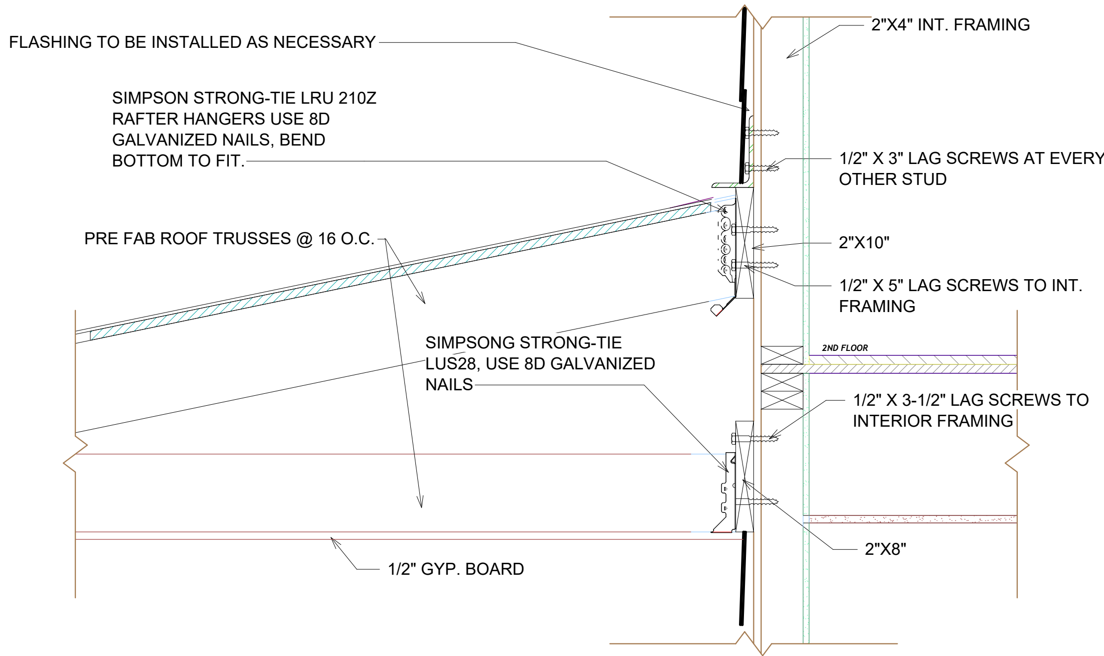
3 ATTACHMENT TO WALL DETAIL 1 1/2" = 1'-0"
