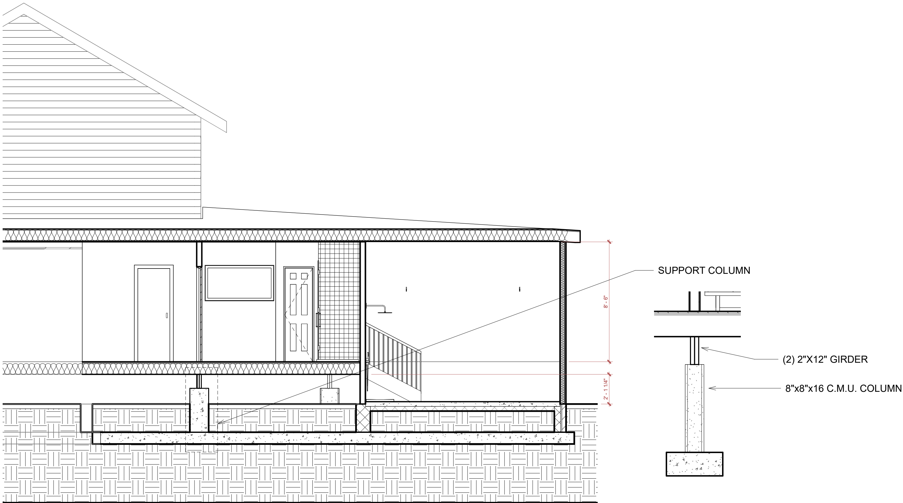
2 Section 2 1/4" = 1'-0"
