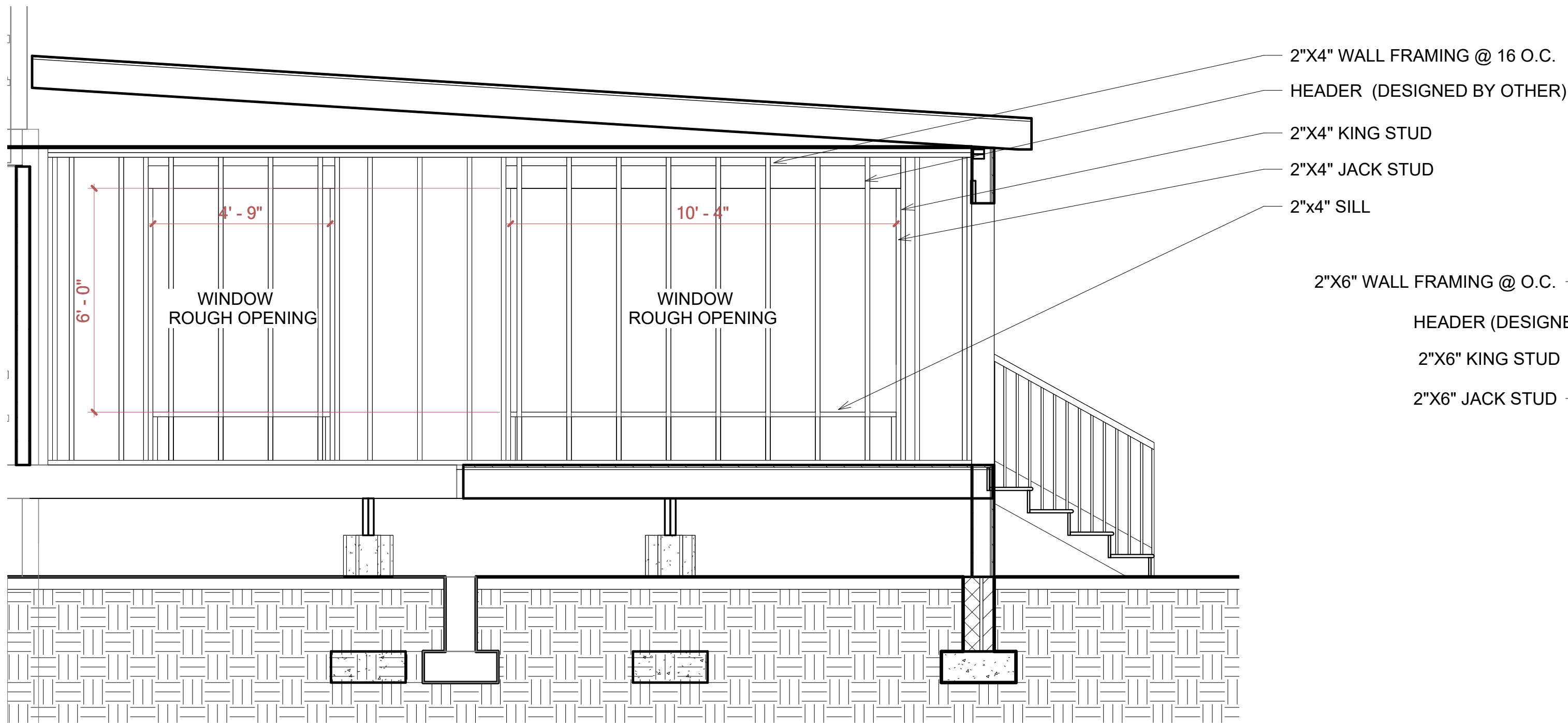
4 LEFT WALL FRAMING DETAIL 3/8" = 1'-0"
