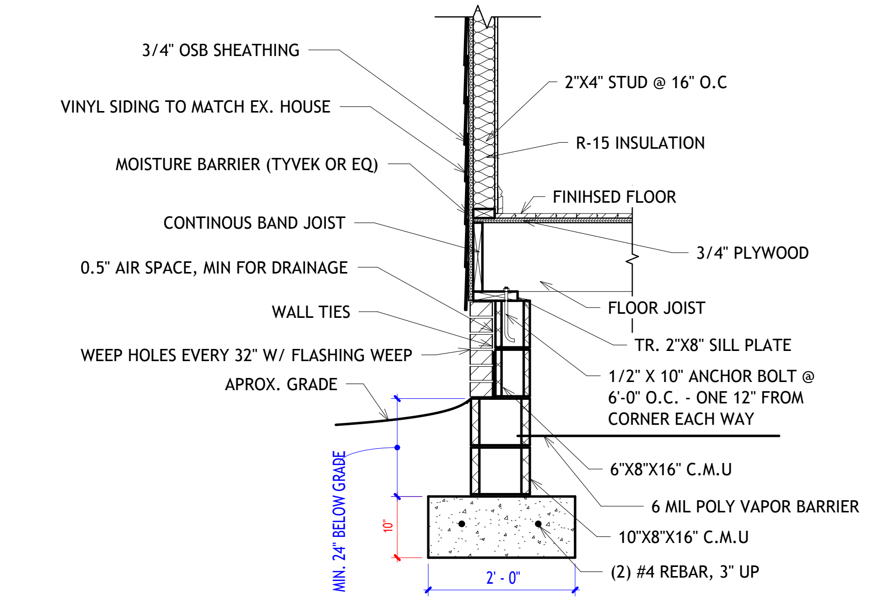
2 FOUNDATION DETAIL 3/4" = 1'-0"
