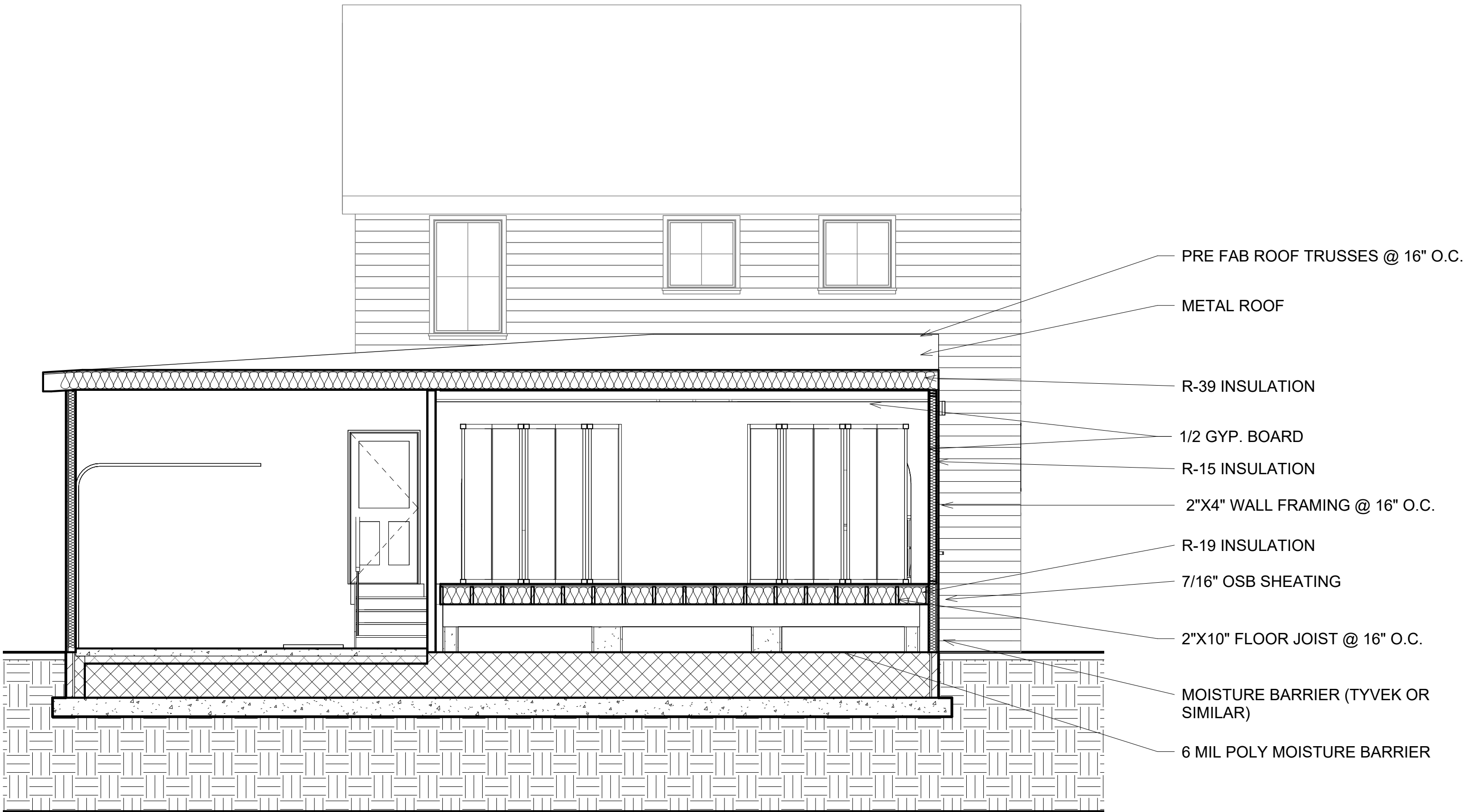
1 Section 1 1/4" = 1'-0"
