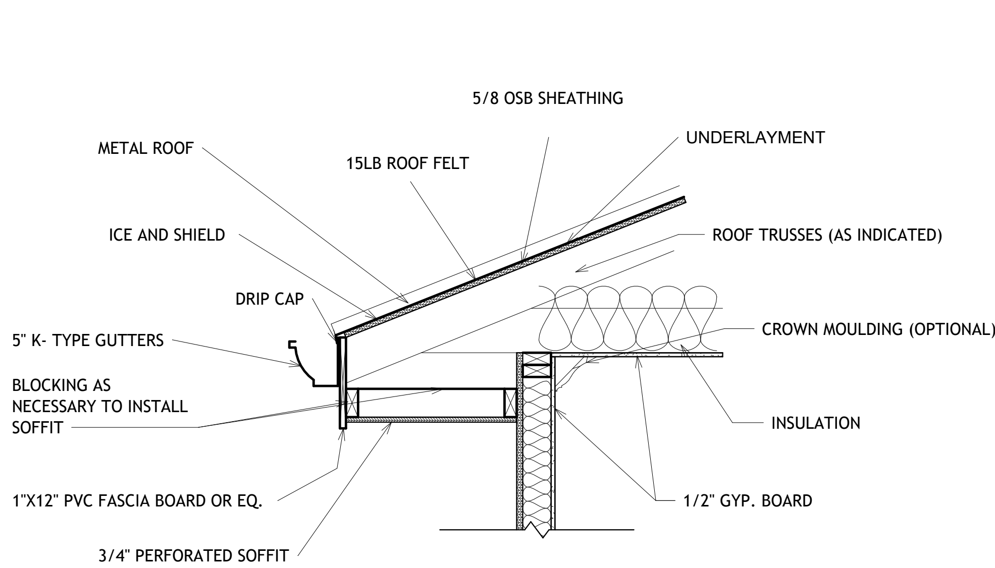
2 TYP SOFFIT DETAIL 1" = 1'-0"
