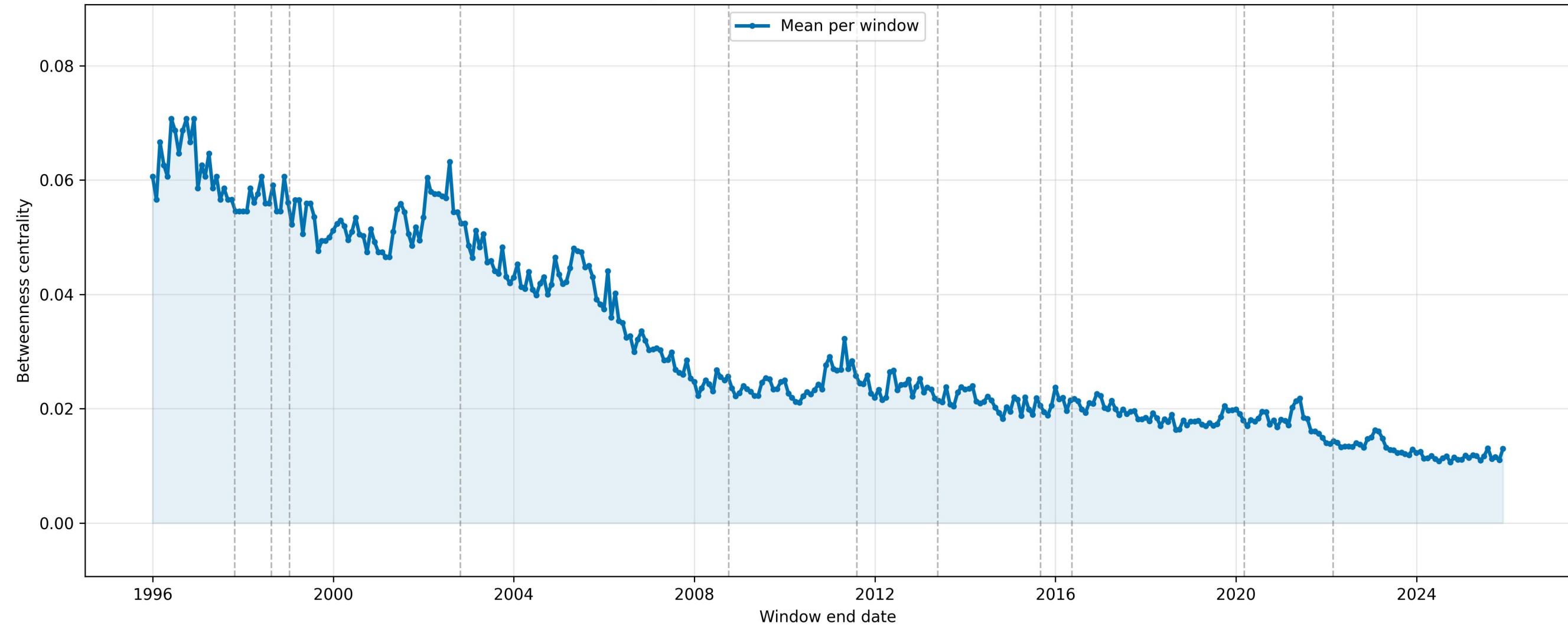
Rolling Betweenness centrality — Planar network
