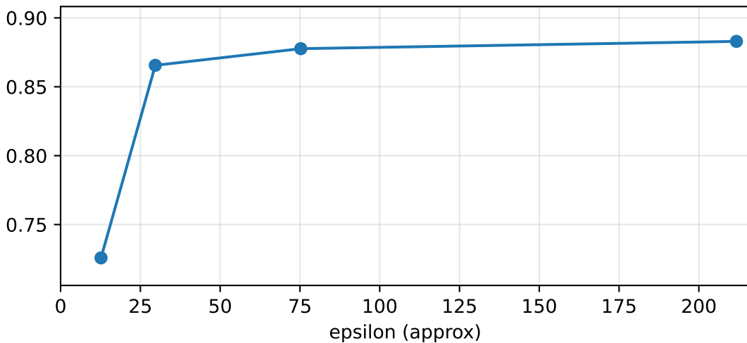
Stage2: private only (DP)
