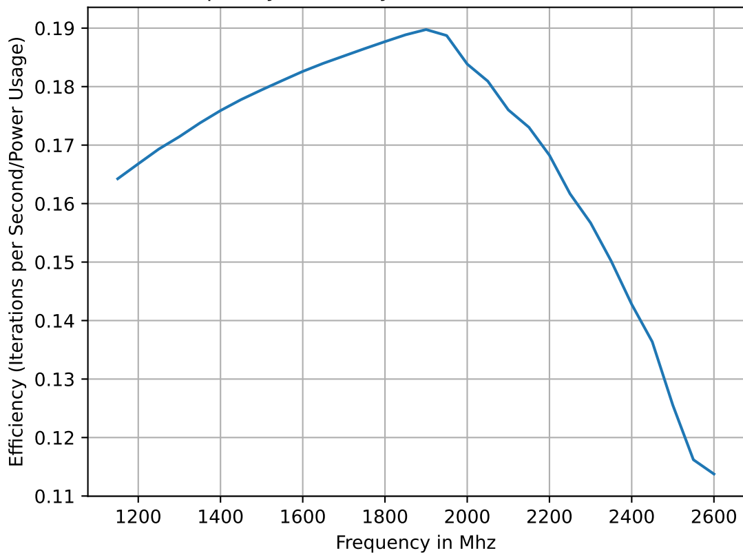
Frequency Efficiency for the AMD RX 6900 XT
