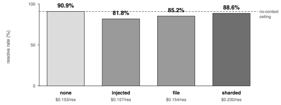
The frontier ceiling: broad-sample delivery matrix Opus 4.8 · 88 random instances · resolve rate; no delivery beats no-context
