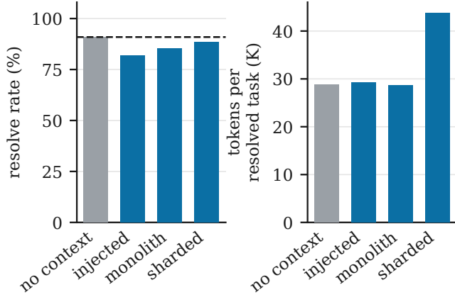
Figure 4: Frontier executor on a broad 88-instance random sample: resolve rate by delivery. No arm exceeds the no-context ceiling (dashed); the sharded store recovers most but at the highest per-resolved cost. Costs are notional, at list prices, excluding prompt caching.
